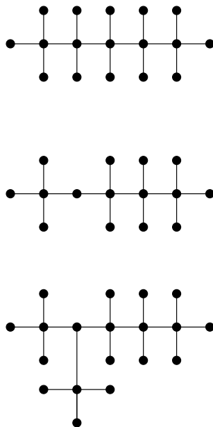
FIGURE 1. Three classes of chemical trees with minimum Randić index
