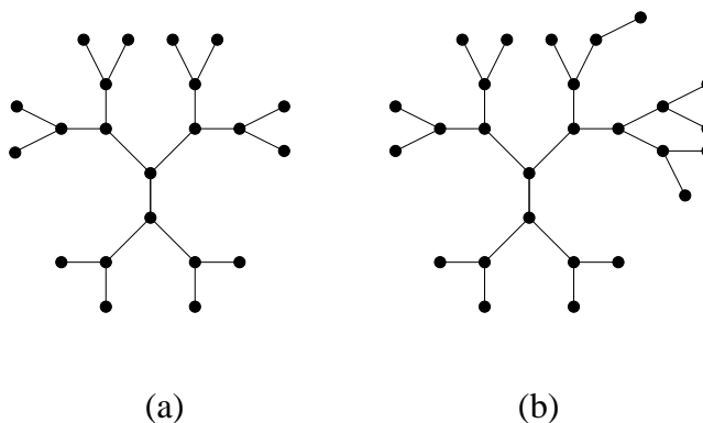
FIGURE 2. Dendrimers without and with additional edges
