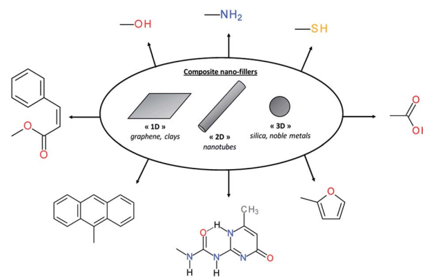
Fig. 12 Different nanofillers based on dimensional aspect and examples of chemical modifications of surface nanofillers for self-healing composites.
