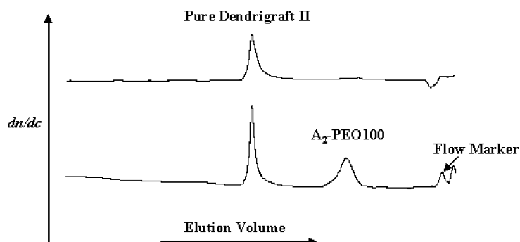
Fig. 2. SEC in water/methanol solvent mixture of dendrigrift II before (bottom) and after selective precipitation (top) of the excess A_2 -PEO100 chains.
