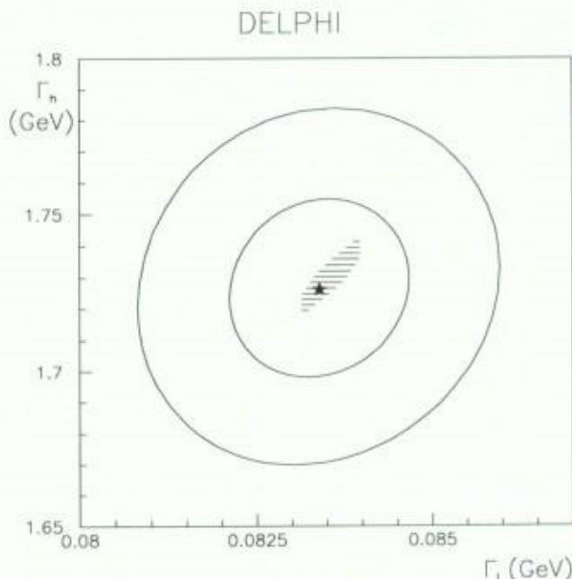
Fig. 15. The 68% and 99% confidence level contours in the \Gamma_h , \Gamma_l plane for the four-parameter fit to the hadronic and leptonic lineshapes. Also shown is the MSM prediction for three massless neutrino species assuming a top-quark mass of 139 \pm 38 GeV, a Higgs mass of 300 GeV, allowed to vary from 50 to 1000 GeV, and a value of \alpha_s of 0.110 \pm 0.006 .
