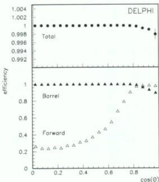
Fig. 4. Trigger efficiency for hadronic events as function of the polar angle of the sphericity axis of the event.
