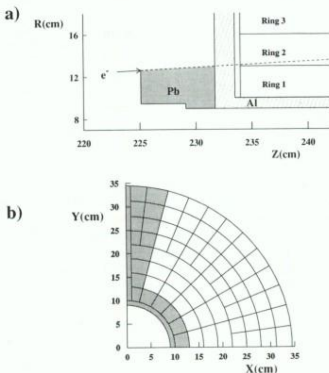
Fig. 2. The Small Angle Tagger calorimeter. (a) Side view showing the lead mask in front of calorimeter. (b) Segmentation in one quadrant. The shaded area indicates the coverage of the mask.
