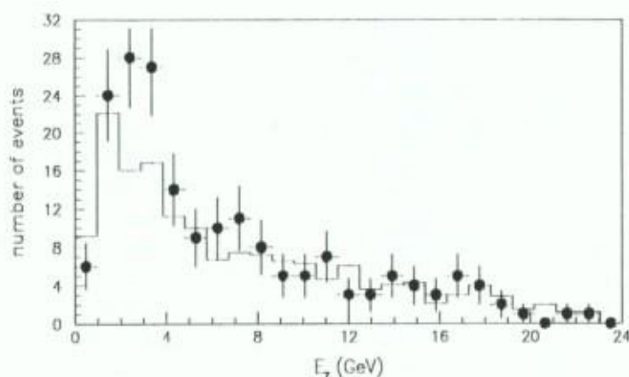
Fig. 6. The photon energy E_\gamma for radiative events in which the transverse energy of the photon with respect to the closest electron is larger than 0.6 GeV. The continuous line is the same distribution for simulated events. The normalisation of the two distributions is based on the relative luminosity of the two samples.
