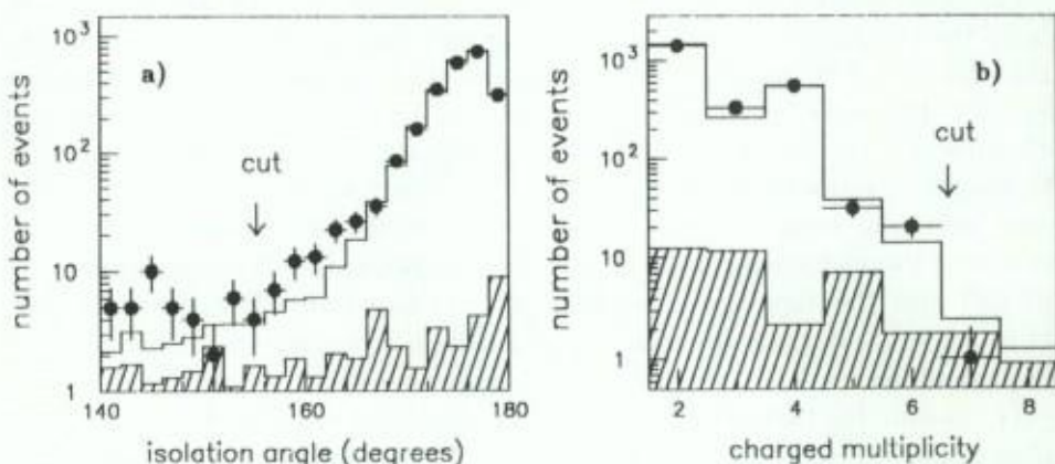
Fig. 10. For events selected in the e^+e^- \rightarrow \tau^+\tau^- analysis: (a) the observed isolation angle distribution superimposed upon the Monte Carlo prediction (solid line) and the estimated background (hatched area); (b) the observed charged track multiplicity distribution superimposed upon the Monte Carlo prediction (solid line) and the estimated background (hatched area). The cut on each of these variables used in the analysis is indicated with an arrow.
