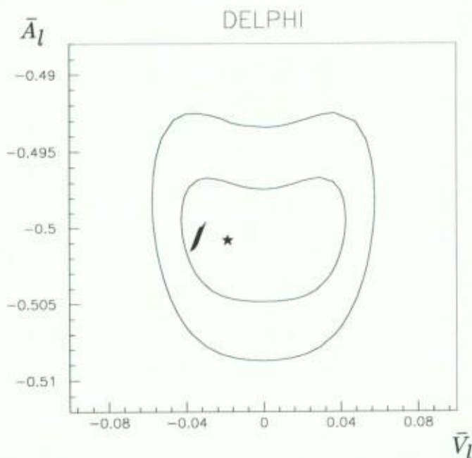
Fig. 17. The 68% and 99% confidence level contours in the \bar{V}_l , \bar{A}_l plane for the five-parameter fit to the e^+e^- \rightarrow e^+e^- ( t -channel subtracted), e^+e^- \rightarrow \mu^+\mu^- , e^+e^- \rightarrow \tau^+\tau^- and e^+e^- \rightarrow \text{hadrons} data displayed in fig. 12, fig. 14 and fig. 16. Also shown is the MSM prediction for three massless neutrino species assuming a top-quark mass of 139 \pm 38 GeV, a Higgs mass of 300 GeV, allowed to vary from 50 to 1000 GeV, and a value of \alpha_s , of 0.110 \pm 0.006 .
