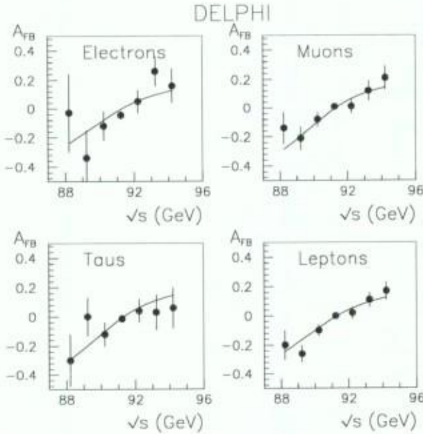
Fig. 16. The forward-backward charge-asymmetries for e^+e^- \rightarrow e^+e^- ( t -channel subtracted), e^+e^- \rightarrow \mu^+\mu^- , e^+e^- \rightarrow \tau^+\tau^- and e^+e^- \rightarrow l^+l^- (flavour-independent analysis, electron t -channel subtracted) as a function of the centre-of-mass energy. The asymmetry data are corrected as described in the text and tables. The curves are the results of a five-parameter fit to the data as described in the text.
