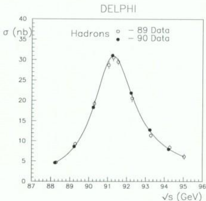
Fig. 12. Cross sections for e^+e^- \rightarrow \text{hadrons} as measured at seventeen different energies. Also shown (solid line) is the result of the three-parameter fit described in the text.
