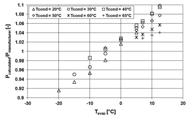
Fig. 3 – P_{\text{calculated}}/P_{\text{manufacturer}} versus T_{\text{evap}} for compressor #5 with R407C.
