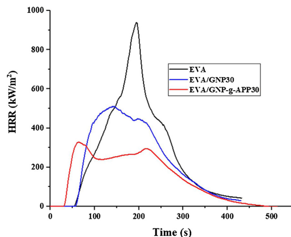
Fig. 13 – HRR curves of pristine EVA and composites (35 kW/m²).
