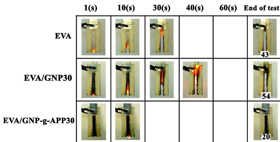
Fig. 10 – Digital photographs of EVA, EVA/GNP30, and EVA/GNP-g-APP30 during and after the vertical burning test.
