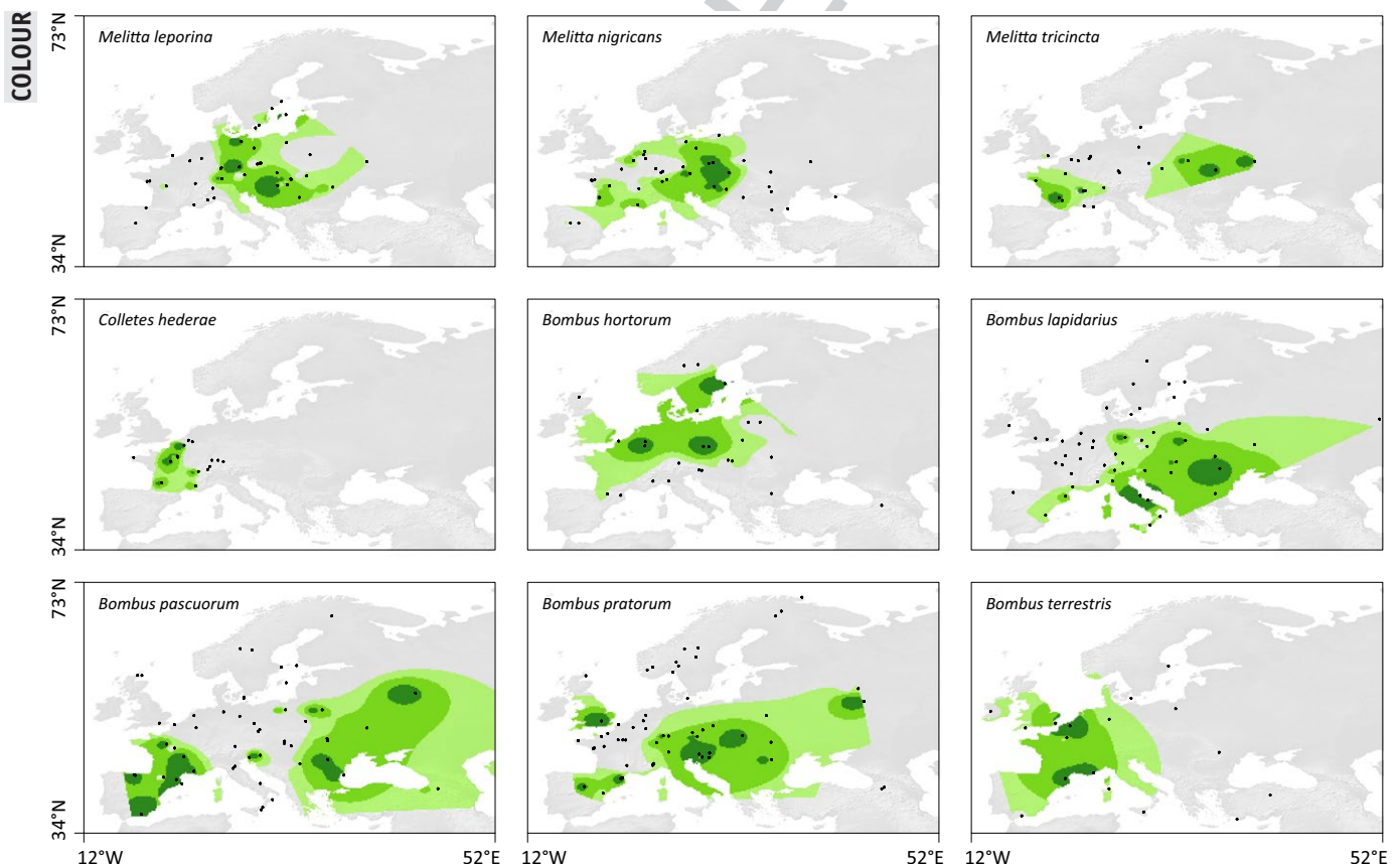
FIGURE 1 For each considered species, areas with nucleotide diversity higher than specific threshold values (0.50, 0.75 and 0.95 quantile values, in shades of increasing darkness). See Material and methods section for a complete description of the method used to generate these surfaces. The black dots are sampled populations with more than two specimens. This figure is based on initial interpolation surfaces based on a sliding window with a radius r = 50 km (see Supporting information Figures S1 and S2 for equivalent figures based on sliding window radius r = 25 and 100 km, and Supporting information Figure S3 for maps displaying variation of genetic diversity among loci)
