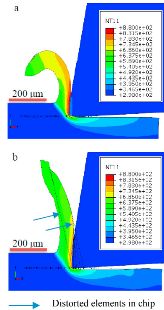
Fig. 9. Temperature contours (in K) of the numerical chip at 1200 \mu s (a) JC-Hou_1 (b) JC-Hou_2.
