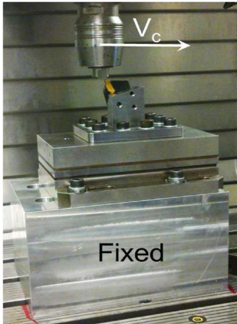
Fig. 5. Cutting configuration on the milling machine [7].
