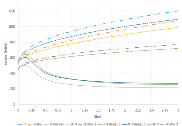
Fig. 3. Stress-strain curves of three constitutive law with three sets of parameters at T=973 K and \dot{\epsilon}_0 = 10\,000 \text{ s}^{-1}
