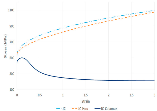
Fig. 2. Stress-strain curves of JC, JC-Calamaz and JC-Hou at T=973 K and \dot{\epsilon}_0 = 10\,000 \text{ s}^{-1}
