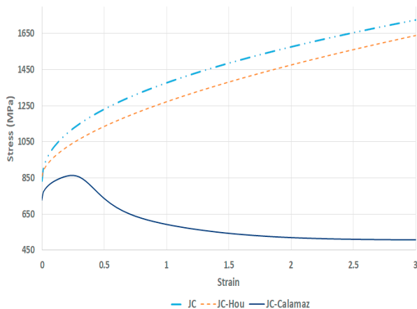
Fig. 1. Stress-strain curves of JC, JC-Calamaz and JC-Hou at T=573 K and \dot{\epsilon}_0 = 10\,000 \text{ s}^{-1}
