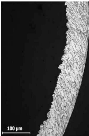
Fig. 6. Experimental reference Chip morphology for uncut chip thickness of 60 \mu\text{m} [7].
