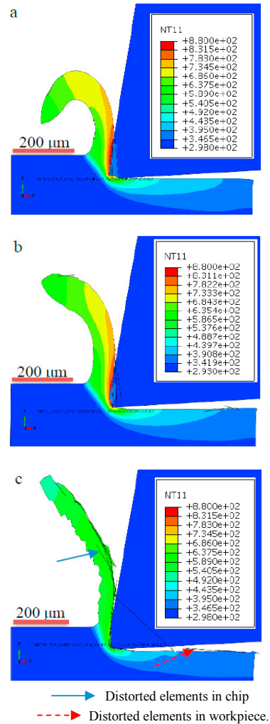
Fig. 7. Temperature contours (in K) of the numerical chip at 1200 \mu\text{s} (a) JC; (b) JC-Hou; (c) JC-Calamaz.
