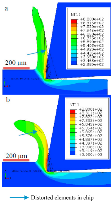
Fig. 8. Temperature contours (in K) of the numerical chip at 1200 \mu s (a) JC_2; (c) JC_3.
