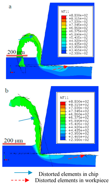
Fig. 10. Temperature contours (in K) of the numerical chip at 1200 \mu s (a) JC-Calamaz_1 (b) JC-Calamaz_3.
