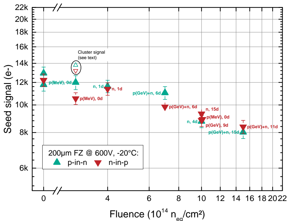
Figure 9. Charge collected on the seed strip for sensors with a nominal active thickness of 200\ \mu\text{m} after a short annealing time of between 0 and 15 days at room temperature. The error bars reflect an estimated uncertainty of about 5% representing statistical and gain uncertainties. The text next to the symbols indicates the irradiation type ( p stands for protons with energy range MeV/GeV and n for neutrons) and the equivalent annealing time at 21\ ^\circ\text{C} .
