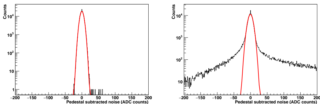
Figure 10. Two examples of pedestal-subtracted noise distributions as measured with the ALiBaVa system and fitted by a Gaussian distribution: a normal noise distribution (left) as observed on p-in-n type FZ sensors before irradiation, which looks similar for n-in-p sensors (both non-irradiated and irradiated), and a noise distribution affected by the non-Gaussian component observed for irradiated p-in-n FZ sensors with a nominal active thickness of 200\ \mu\text{m} (right).
