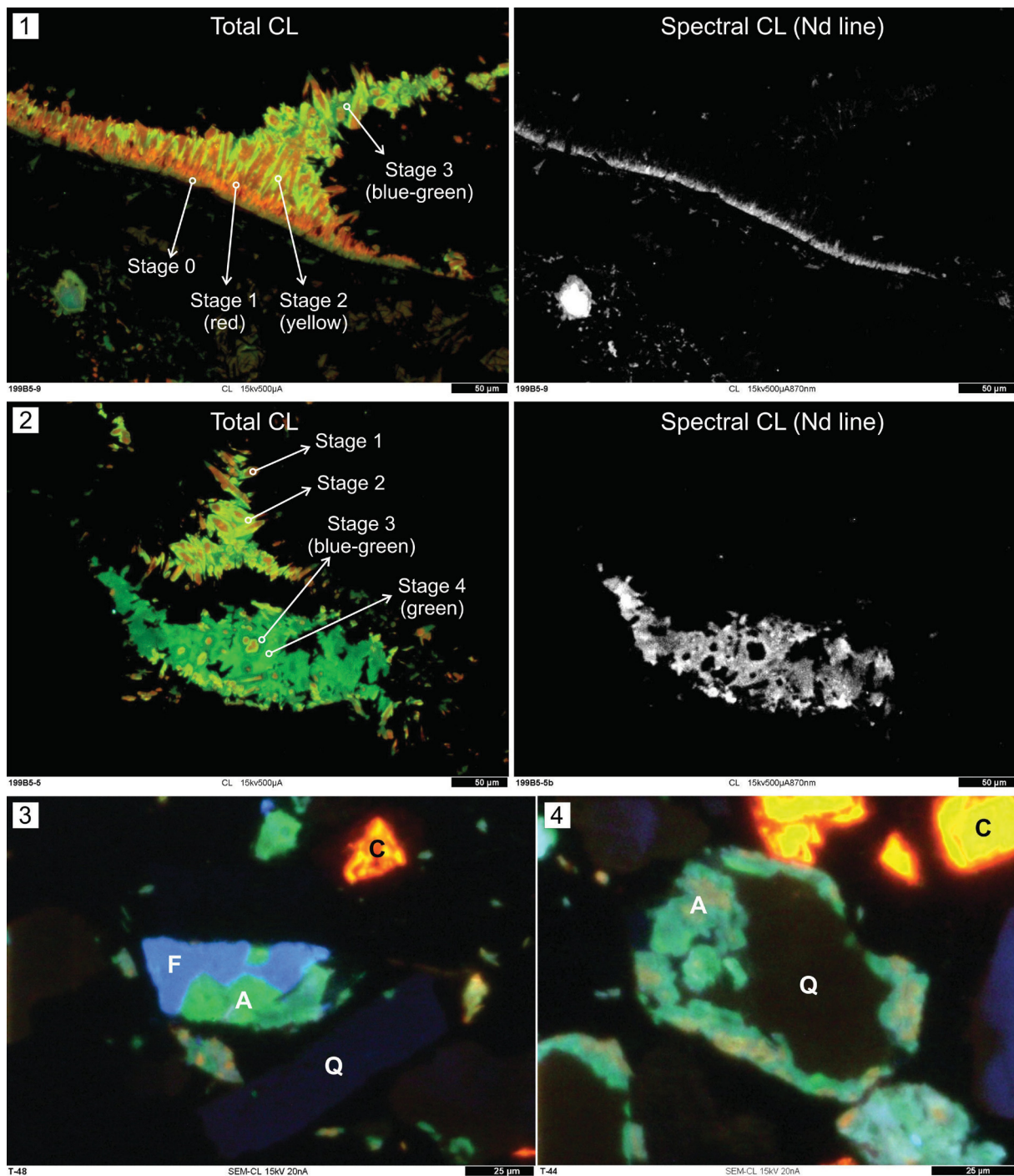
Fig. 2 – Cathodoluminescence imaging of apatite in the Saint-Ghislain ironstone. Photos 1 and 2 depict the diagenetic sequence in total (left) and spectral (right) CL (optical CL, scale bar 50 μm). The latter show the distribution of neodymium, which is not visible in total CL because it occurs in the near-infrared. In photos 3 and 4, apatite is replacing feldspars and quartz grains (SEM-CL, scale bar 25 μm). F = feldspar, Q = quartz, A = apatite and C = calcite.
