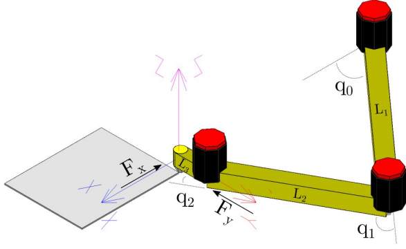
Fig. 8: Fanuc robot model
