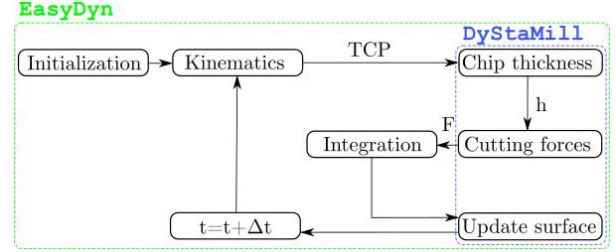
Fig. 6: Solving of the coupled dynamic system
