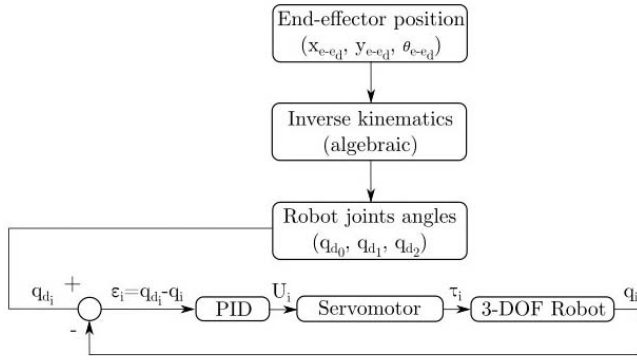
Fig. 10: Inverse kinematics and joints controllers
