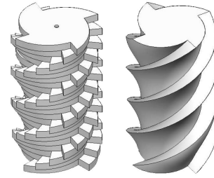
Fig. 4: Axial tool discretization
