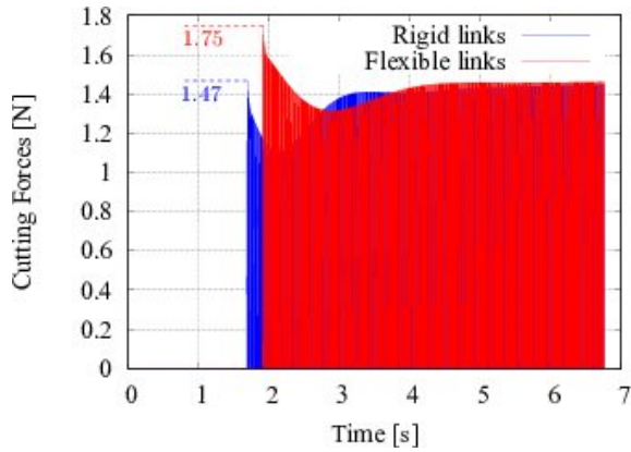
Fig. 19: Cutting forces (+spring)
