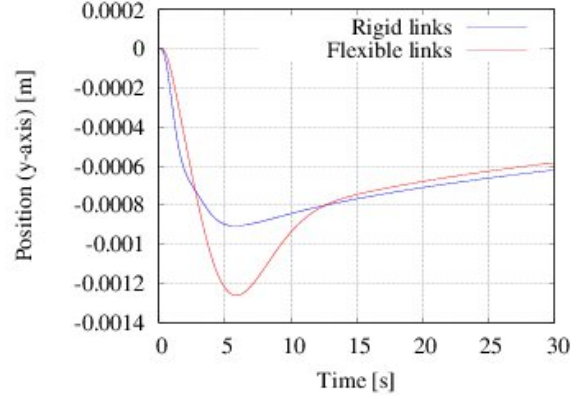
Fig. 12: Tracking along y-axis without machining
