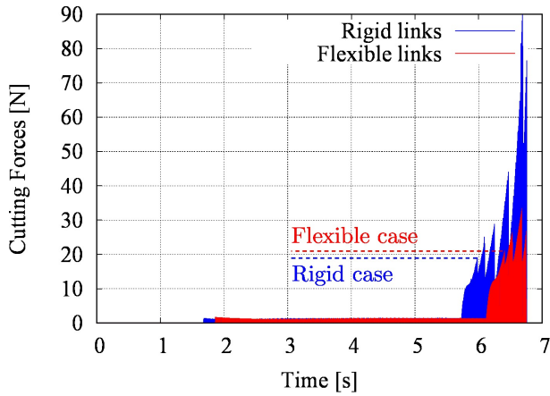
Fig. 13: Cutting forces
