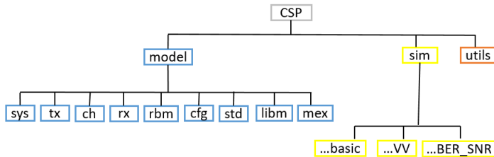
Fig. 5. Top-level directory structure (adapted from [17]).
