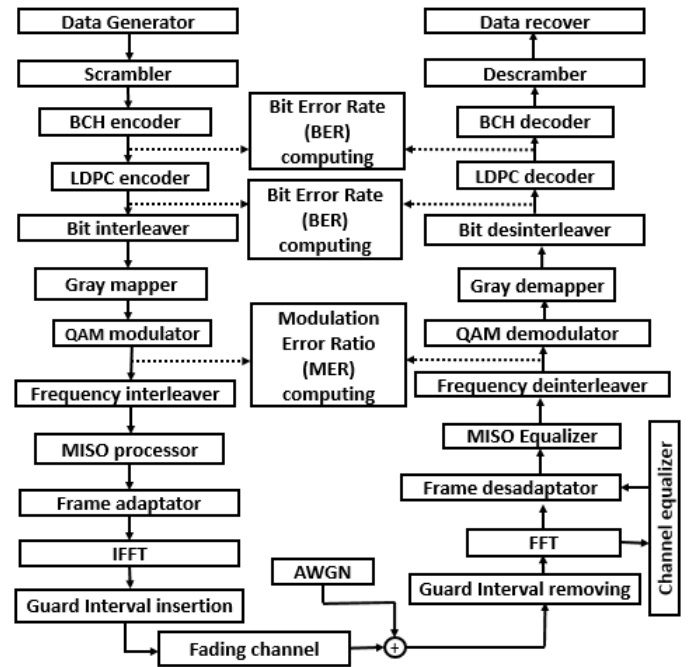
Fig. 6. System implemented.
