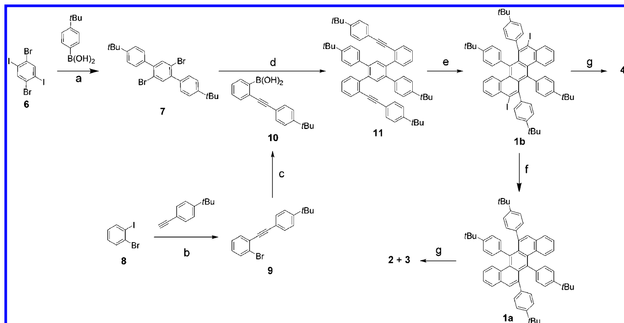
Scheme 3. Synthesis of PAHs 2, 3, and 4 a
