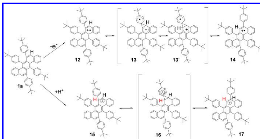
Scheme 4. Comparison between Radical Cation and Arenium Cation Mechanisms for the 1,2-Shift of the Aryl Groups
