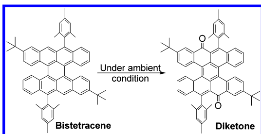
Scheme 1. Oxidation of Bistetracene to a Diketone under Ambient Conditions
