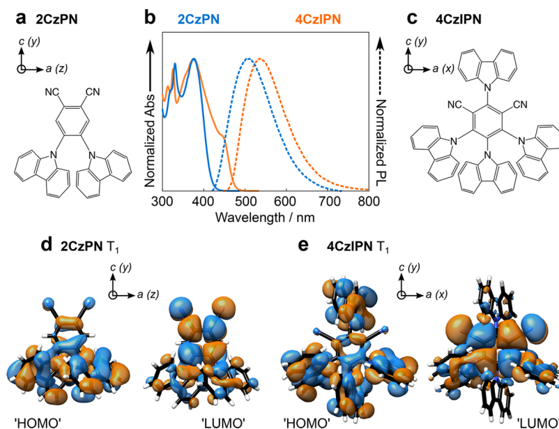
Figure 1. Chemical structures for (a) 2CzPN and (c) 4CzIPN. (b) UV–vis absorption (abs) and photoluminescence (PL) spectra for 100 \mu\text{M} 2CzPN (blue)/4CzIPN (orange) in toluene. UKS-DFT-calculated canonical orbitals for the T_1 states of (d) 2CzPN and (e) 4CzIPN, using the PBE0 functional and EPR-II basis set. a , b , and c and x , y , and z denote the symmetry and ZFS axes, respectively.
