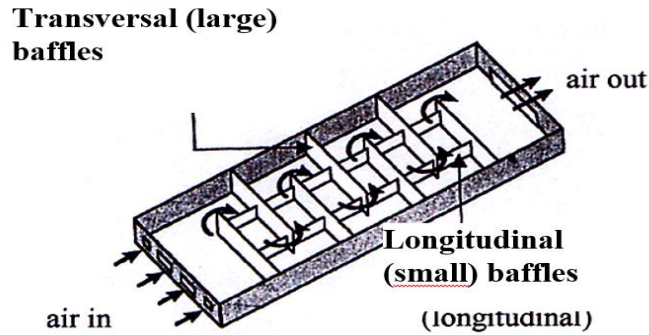
Figure 7 Solar panel equipped with TL type baffles
