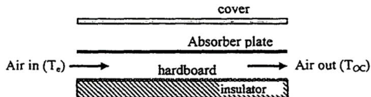
Figure 2 Solar air fiat plate collector without obstacles
