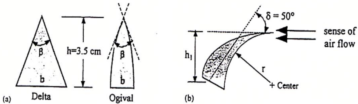
Figure 5 Delta and ogival baffles (a) before bending; (b) after bending
