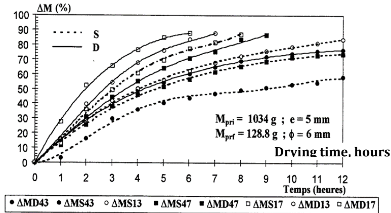
Figure 9 Evolution of the loss of mass ( \Delta M ) of plums in relation to drying time measured at the first and fourth trays with flows of 31.3\text{m}^3/\text{h.m}^2 and 70\text{m}^3/\text{h.m}^2 using DCL1 and TL type solar panels, data recorded on a typical July day at the Valenciennes site.
