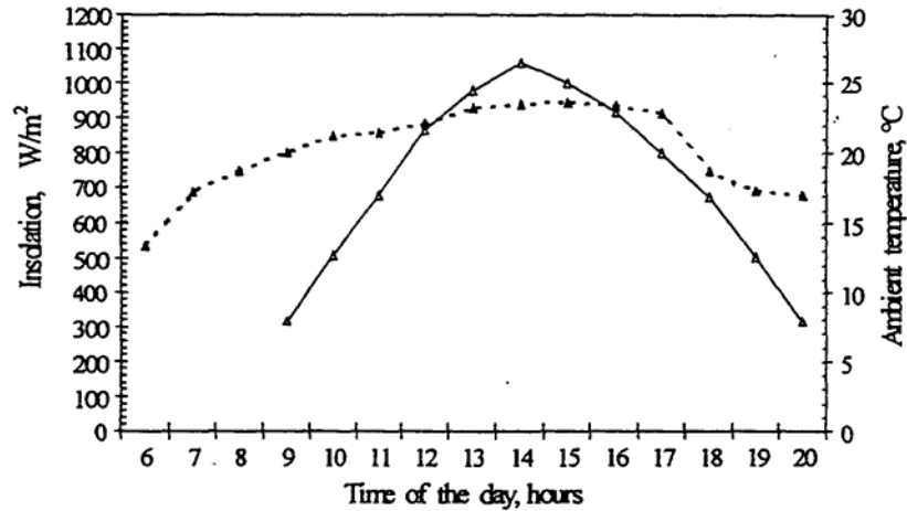
Figure 3 Variation of the ambient temperature and the insolation during the characteristic day of July, at Valenciennes -8-glob:1J hourly insolation (/cs); " ambient temperature (T.).
