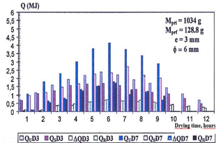
Figure 12 Variations in quantities of heat (Q) in relation to drying time with flows of 31.3\text{m}^3/\text{h.m}^2 and 70\text{m}^3/\text{h.m}^2 using an WB type solar panel (without baffles)
