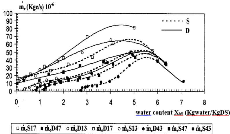
Figure 11 Evolution of the drying speed ( m_e ) in relation to water content to the point when the product is completely dried with flows of 31.3\text{m}^3/\text{h.m}^2 and 70\text{m}^3/\text{h.m}^2 using WB and DCL1 type solar panels
