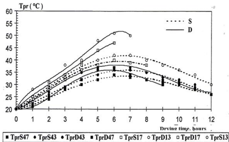
Figure 10 Evolution of the temperature of GINGER in relation to drying time measured at the first and fourth trays with flows of 31.3\text{m}^3/\text{h.m}^2 and 70\text{m}^3/\text{h.m}^2 using WB, DCL1 and TL type solar panels
