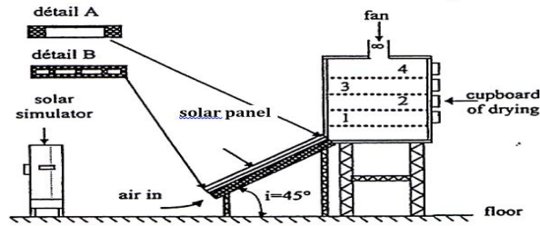
Figure 1 Experimental Device
