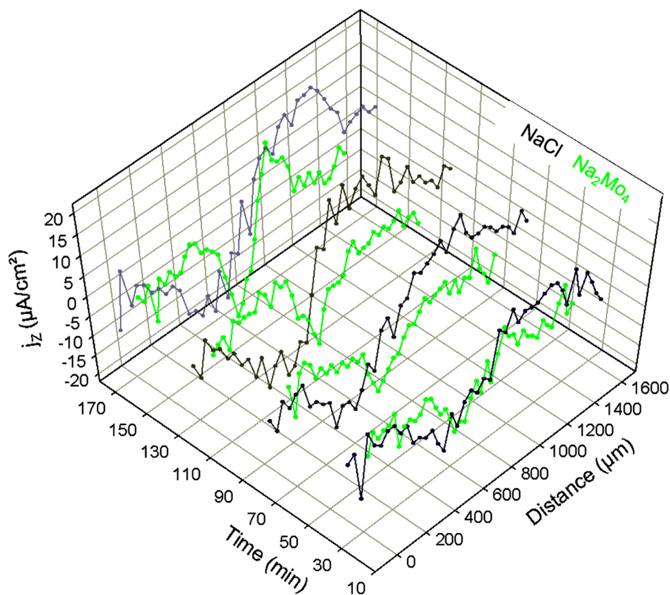
Fig. 14. j_z line profiles constructed from the 4 consecutive SVET scans obtained in 0.05 M NaCl or 0.05 M NaCl + 5 mM \text{Na}_2\text{MoO}_4 during 180 min. The directions considered are indicated by lines r-r' (Fig. 10(b)) and i-i' (Fig. 13(b)) for the reference and the inhibitive solution, respectively.
