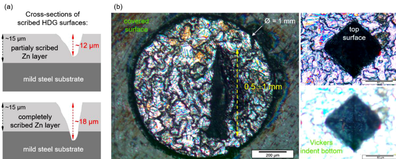
Fig. 3. (a) schematic illustration of the two types of scribed HDG surfaces analysed by SVET: scratches with ~12 or ~18 μm in depth (partial or complete removal of the Zn-rich layers, respectively) (b) schematic representation of the optical microscopy method employed for estimating defect depths: the distances between Vickers indent bottoms and their top-surfaces (~12 or ~18 μm) were used as references for selecting scratches with ~12 or ~18 μm in depth.
