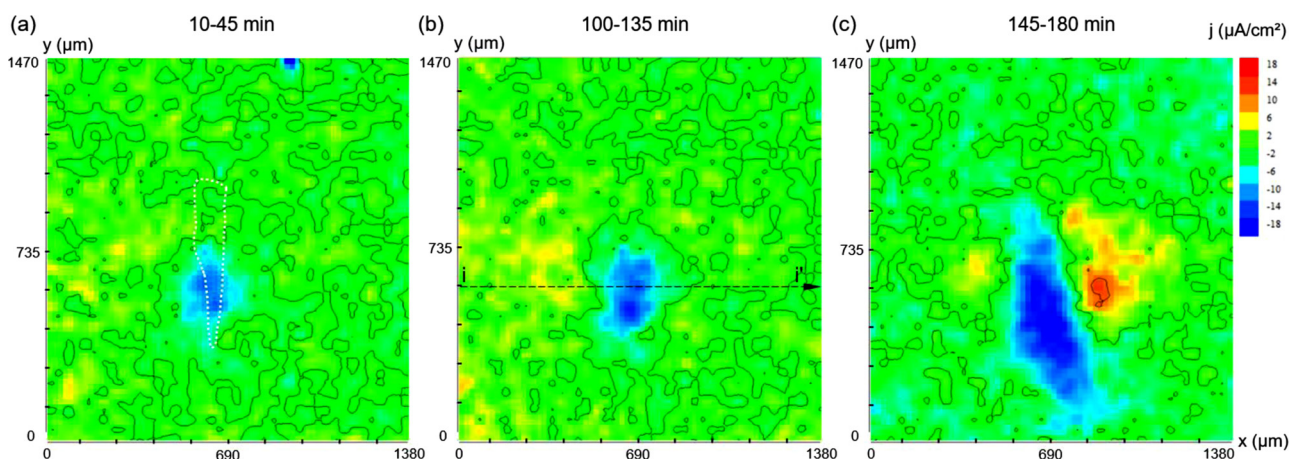
Fig. 13. Current density ( \mu\text{A}/\text{cm}^2 ) maps obtained by SVET on severely scratched HDG (~18 \mu\text{m} -depth defect) exposed to 0.05 M NaCl + 5 mM Na 2 MoO 4 solution after (a) 10–45 min, (b) 100–135 min and (c) 145–180 min of immersion. The j scale is the same for all maps. The scratched zone is represented by white dots in (a). The i-i' line in (b) indicates the direction used for constructing j_z line profiles.
