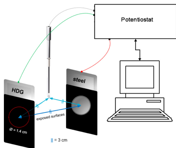
Fig. 2. Schematic representation of the HDG/mild steel galvanic coupling configuration for ZRA testing. The area ratio of the exposed surfaces ( \sim 1.5 \text{ cm}^2 ) was equal to 1.
