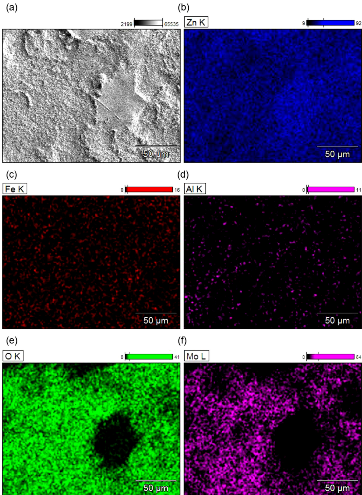
Fig. 7. SEM-EDX analysis of the HDG surface from galvanic couple model after ZRA testing (180 min of immersion in 0.05 M NaCl + 5 mM \text{Na}_2\text{MoO}_4 electrolyte). (a) Secondary electron image. (b, c, d, e, f) Corresponding EDX elementary maps of Zn, Fe, Al, O and Mo.
