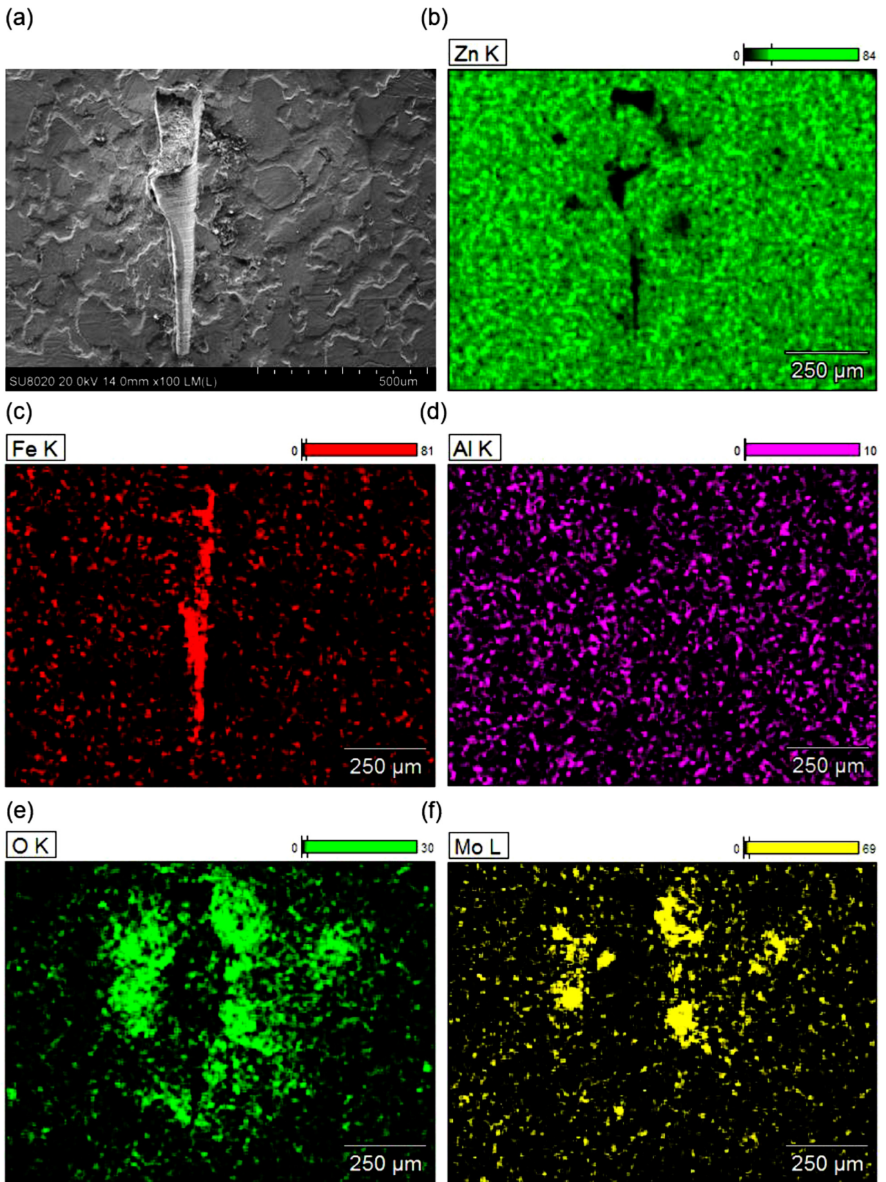
Fig. 15. SEM-EDX analysis of the severely scribed HDG surface after 180 min of immersion in 0.05 M NaCl + 5 mM Na 2 MoO 4 electrolyte. (a) Secondary electron image. (b, c, d, e, f) Corresponding EDX elemental maps of Zn, Fe, Al, and O and Mo.
