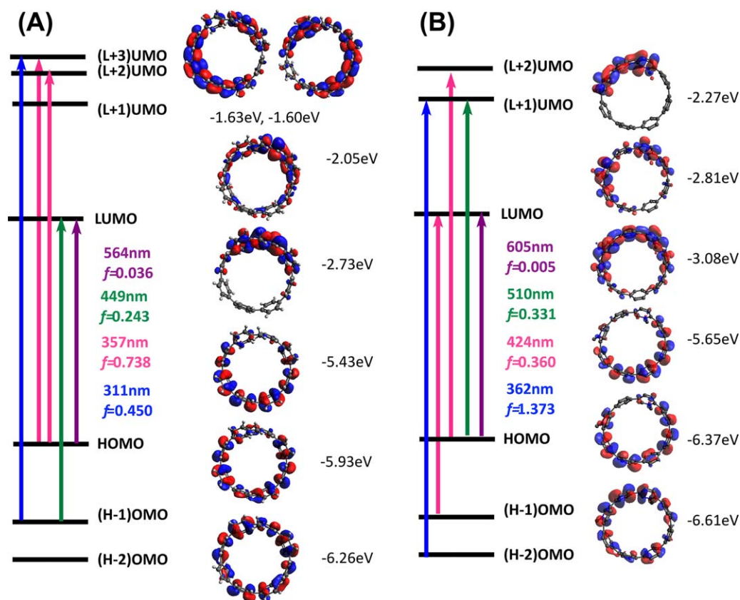
FIGURE 8 Major orbital transitions, arising from the HOMO-2 to the LUMO+2 window of orbitals, for the: (A) N -methylaza-[8]CPP + 7 , and (B) N,N -dimethyl-1,15-diaza-[8]CPP 2+ 8 systems, calculated at the TDA-B3LYP/6-31G* level
