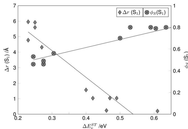
FIGURE 9 Interplay between the calculated \Delta r (in Å) and \phi_S values, and the \Delta E_v^{ST} (in eV) energy difference, at the TDA-PBE0/def2-TZVP level. The solid lines are a guide to the eye
