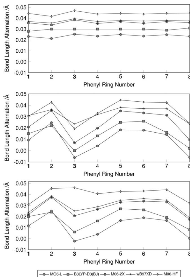
FIGURE 4 Bond Length Alternation (BLA, in Å), calculated as BLA = \frac{1}{2} [(r_1 + r'_1) - (r_2 + r'_2)] , along the phenyl rings of (top) 1,15-diaza[8]CPP 2 , (middle) H,H-1,15-diaza-[8]CPP 2+ 6 , and (bottom) N,N-dimethyl-1,15-diaza-[8]CPP 2+ 8 , calculated at various levels of theory and with the 6-31G* basis set. The phenyl rings 1 and 3 carry the nitrogen functionality in all cases
