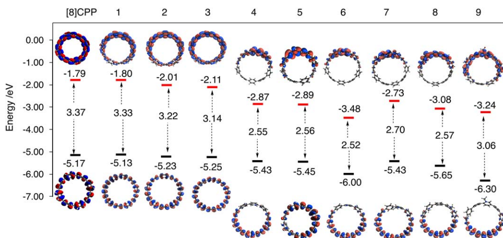
FIGURE 5 From left to right: Isocontour plots and energy values (in acetonitrile) of the HOMO and LUMO orbitals for [8]CPP and the set of N-doped CPPs 1 to 9 . Red and blue for positive and negative signs of the lobes. All values obtained from the optimized geometries at the B3LYP-D3(BJ)/6-31G* level
