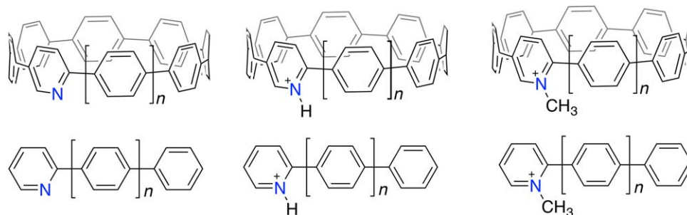
FIGURE 6 From left to right: Increasingly longer cyclic (top) and linear (bottom) N-substituted nanohoops aza-[ n ]CPP, H-aza-[ n ]CPP + , and N-methylaza-[ n ]CPP +
