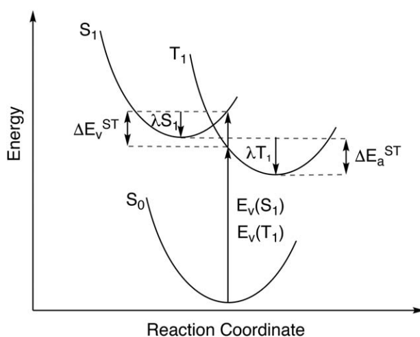
FIGURE 3 Sketch of the main excited-states processes studied along this work. Note that the curves for the S_1 and T_1 excited-states are exaggeratedly shifted for the sake of clarity
