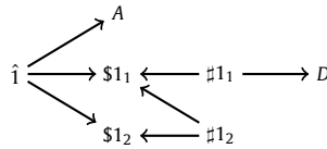
Fig. 5. For any structure (\mathcal{D}, \mathcal{S}, \sigma, \gamma) whose membership relation contains the pairs visualized above, \text{BiToTer}(\mathcal{D}, \mathcal{S}, \sigma, \gamma) contains (A, D, D) .
