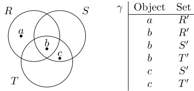
Fig. 2. Encoding of a finite sequence of sets by a binary membership relation.
