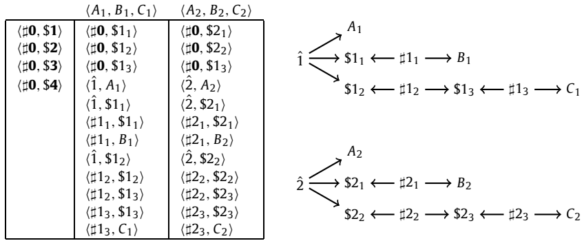
Fig. 4. The ternary relation I = \{\langle A_1, B_1, C_1 \rangle, \langle A_2, B_2, C_2 \rangle\} translated to a binary relation.
