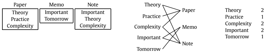
Fig. 1. Left, a sequence of documents. Middle, the same dataset represented as a bipartite graph. Right, the frequency of words in this data set.
