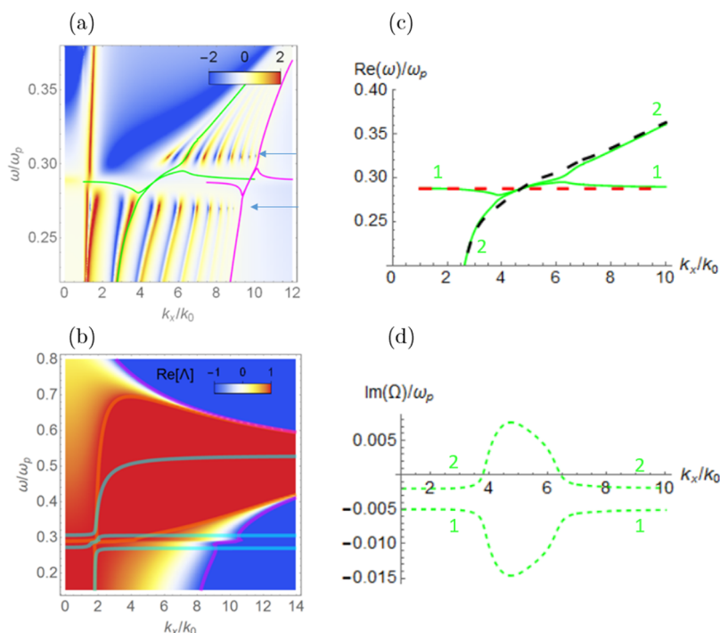
Figure 4. (a) Reflectance with an emission line in the large coupling strength regime ( g_e = 10^{14} ) for the finite structure (logarithmic scale). The green and magenta curves were obtained via our semiclassical model on two different modes. (b) Dispersion diagram of the infinite structure with an emission line in the large coupling strength regime. Orange curves are the edges of the plasmonic band at the center of the Brillouin zone ( \text{Re}(\Lambda) = 1 ), magenta curves are those at the edge of the Brillouin zone ( \text{Re}(\Lambda) = -1 ), and cyan curves are the loss-compensation boundary ( \text{Im}(\Lambda) = 0 ). (c) Real (green solid curves) and (d) imaginary (green dashed curves) parts of the complex eigenfrequencies \Omega_{\pm} obtained with our semiclassical model. In (c) the red dashed curve is the excitonic emission line and the black dashed curve is the unperturbed optical mode. The two polaritons resulting from the coupling of the optical mode with the excitonic line are identified by the green numbers 1 and 2 ( \Omega_+ and \Omega_- , respectively).
