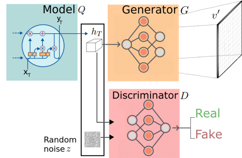
Figure 2: Training flow of Q -WAAE. The last hidden state h_T is the input for decoder P
