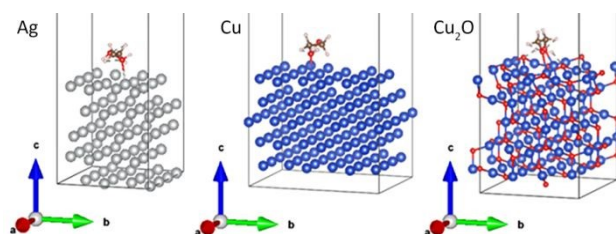
Figure 11 Relaxed interface geometries of EG onto Ag(111), Cu(111), and Cu 2 O(111) surfaces.
