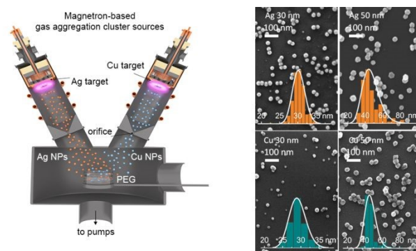
Figure 1 Left: scheme of experimental setup for simultaneous deposition of Cu and Ag NPs into PEG using two independent gas aggregation cluster sources. Right: SEM images of Ag and Cu NPs deposited with different mean size on Si substrates. Insets show the size distributions. The deposition parameters are given in Table 1.
