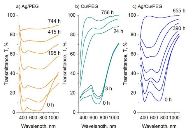
Figure 4 Time evolution of the UV-Vis transmittance spectra of: a) Ag/PEG, b) Cu/PEG, and c) Ag/Cu/PEG nanofluids. The NP mean size is 30 nm, the total metal concentration is 50 \mu\text{g}/\text{mL} (25 \mu\text{g}/\text{mL} of Ag and 25 \mu\text{g}/\text{mL} of Cu, in the case of Ag/Cu/PEG).
