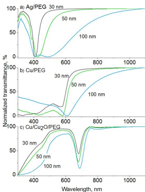
Figure 7 Simulated UV-Vis transmittance spectra of: a) Ag/PEG, b) Cu/PEG, and c) Cu/Cu 2 O/PEG nanofluids with NPs of different mean size. The NPs are distributed lognormally with standard deviation of 20%. For core/shell Cu/Cu 2 O NPs, the radius of the Cu core is equal to the thickness of the Cu 2 O shell. The spectra are normalized to the range 0 to 100%.
