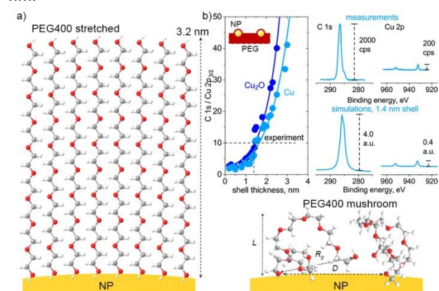
Figure 13 a) Two types of PEG400 configuration on the NP surface: high-density brush and low-density mushroom arrangements; b) SESSA simulations of XPS C 1s and Cu 2p spectra with different thickness of PEG shell over Cu or Cu 2 O NPs; the simulations are compared with the XPS spectra measured on Cu/PEG nanofluid by enviro-ESCA. 26
