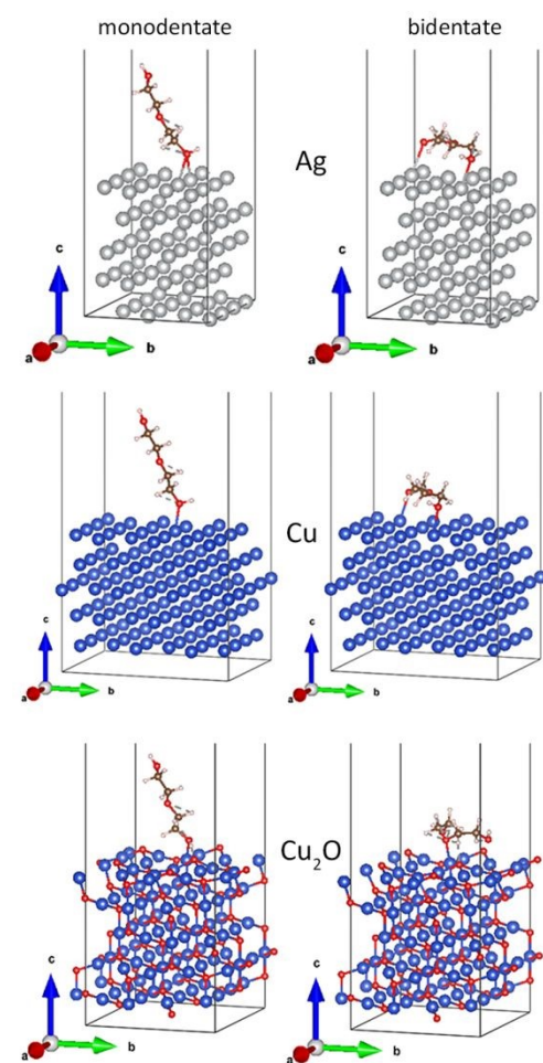
Figure 12 Relaxed interface geometries of DEG onto Ag(111), Cu(111), and Cu 2 O(111) surfaces. Left column: monodentate configuration, right column: bidentate configuration.
