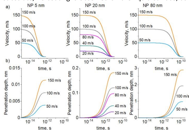
Figure 2 CFD simulation of a single 5, 20, or 80 nm Cu NP retarding from the initial velocity to zero when moving in PEG: a) NP velocity; b) NP penetration depth.
