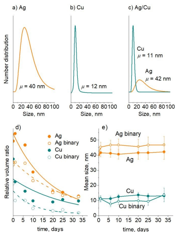
Figure 9 In-liquid SAXS results obtained on single-metal Ag/PEG, Cu/PEG, and binary Ag/Cu/PEG nanofluids: a)-c) number-weighted size distributions; d) attenuation of the scattering intensity in time, lines as guides for the eye; e) the evolution of the mean NP size in time. The initial total metal concentration is 50 \mu\text{g/mL} (25 \mu\text{g/mL} of Ag and 25 \mu\text{g/mL} of Cu, in the case of Ag/Cu/PEG).
