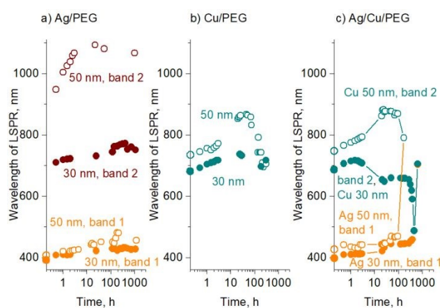
Figure 6 Change in the LSPR position with time for nanofluids with NPs of mean size of 30 and 50 nm: a) Ag/PEG, b) Cu/PEG, and c) Ag/Cu/PEG. The total metal concentration is 50 µg/mL (25 µg/mL of Ag and 25 µg/mL of Cu, in the case of Ag/Cu/PEG). Data points placed on the y-axes belong to time = 0 h.
