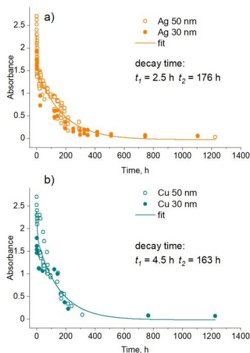
Figure 8 Attenuation of LSPR absorbance maxima with time for NPs of 30 and 50 nm mean size during their sedimentation: a) Ag; b) Cu. The total metal concentration is 50 \mu\text{g}/\text{mL} . The lines are fits by a two-exponential decay.
