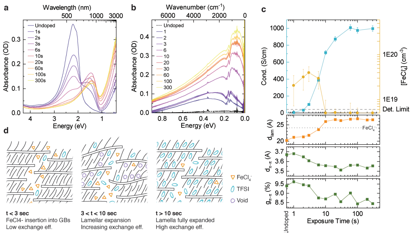
Figure 4. Kinetics of ion exchange doping. Doping solutions consisted of 100/1 \times 10^{-3} M BMP TFSI/FeCl 3 in AN. a) UV-vis-NIR spectra. b) FTIR spectra. c) Electrical conductivity, residual FeCl 4 - (extracted from UV-vis spectra), unit cell parameters, and \pi - \pi paracrystallinity (extracted from GIWAXS data) as a function of doping time. d) Illustration of film microstructure at different doping times.
