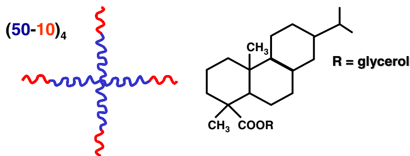
Scheme 1. Sketch of (left) the "all-acrylate" star copolymer. This star copolymer is denoted as (A-B) 4 where A and B represent the elastomer segment ( A = P(2EHA-co-MA) = poly(2\text{-ethylhexyl acrylate-co-methyl acrylate}) ) and the thermoplastic segment ( B = PMMA = poly(\text{methyl methacrylate}) ), respectively. (right) the tackifying resin, which is a hydrogenated rosin glycerol ester.
