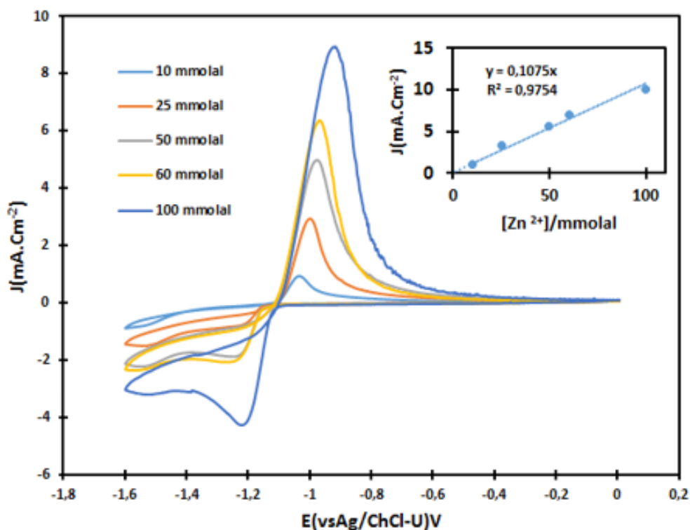
Figure 2. Cyclic voltammograms (3rd cycle) of the ChCl-U system on GC with different concentrations of ZnSO_4 \cdot 7H_2O , v = 10 \text{ mV s}^{-1} , T = 100^\circ\text{C}
