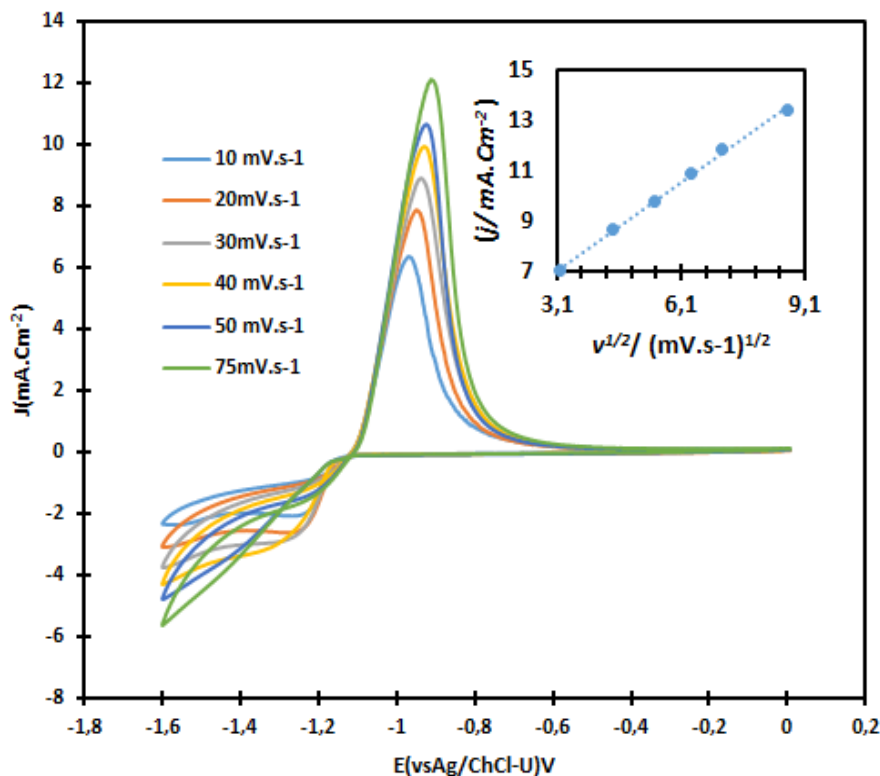
Figure 4. Cyclic voltammograms of ChCl-U + 50 mmol ZnSO 4 .7H 2 O on GC electrode at different scan rate; T=100°C.
