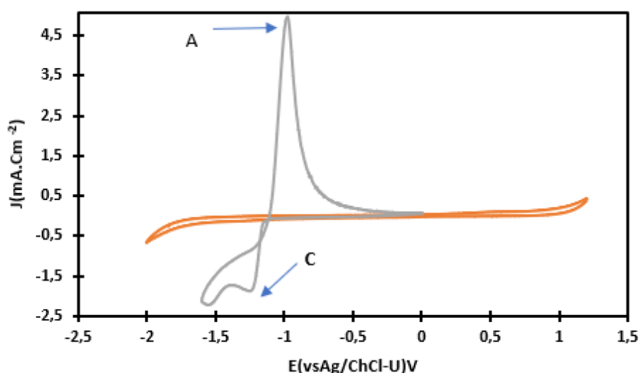
Figure 3. Cyclic voltammogram of the ChCl-U system + 50 mmol of ZnSO_4 \cdot 7H_2O , GC electrode, V = 10 \text{ mV/S} , T = 100^\circ\text{C} .
