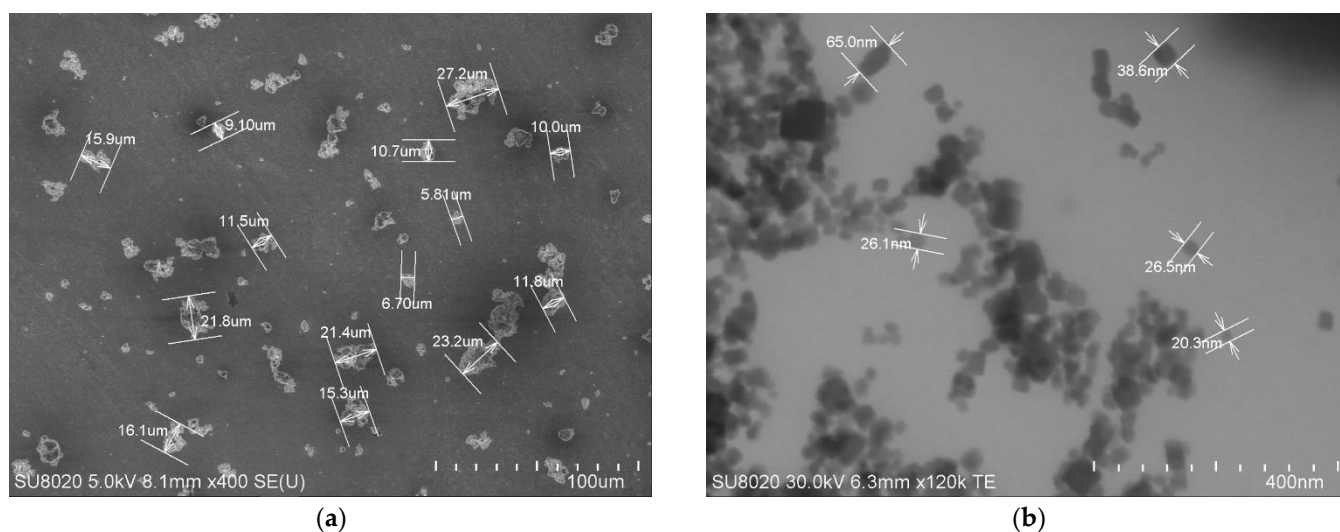
Figure 1. (a,b). Selected images of AHP before and after grinding: (a) SEM of as-received microparticles before grinding; (b) STEM of nanoparticles obtained by the two successive grindings.
