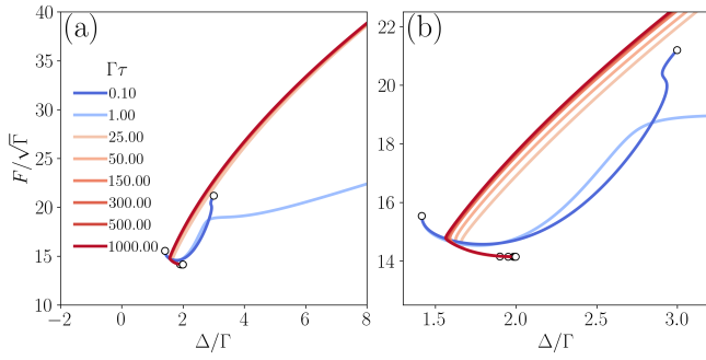
FIG. 8. (a) Hopf bifurcation on the asymmetric branches in the (\Delta, F) -space for various memory times \tau when the coupling is J = 0.5\Gamma . (b) Close-up view on the limit behavior when \Gamma\tau \gg 1 . Model parameters are as in Fig. 5.
