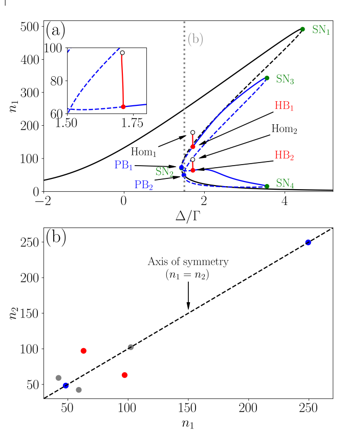
FIG. 5. (a) Bifurcation diagram of n_1 along the detuning \Delta for coupled and symmetrically driven cavities. Solid (dashed) curves represent stable (unstable) fixed points with symmetric and asymmetric solutions in black and blue, respectively. Saddle-node (SN, green), Hopf (HB, red), homoclinic (Hom, black) and pitchfork (PB, blue) bifurcations are located with green, red, empty, and blue dots, respectively. Inset: close-up view of Hopf ( \text{HB}_1 ) and homoclinic ( \text{Hom}_1 ) bifurcations in the main panel. The red solid curve represents the maximum intensity of the stable limit cycle. (b) Fixed points for a detuning \Delta = 1.5\Gamma color coded as in Fig. 2. The dashed black line shows the axis of symmetry n_1 = n_2 . Model parameters: \Gamma = 1 , U = \Gamma/100 , \kappa_L = \Gamma/2 , D = 0 , J = 0.5\Gamma , F = 15.7\sqrt{\Gamma} , \tau = 100\Gamma^{-1} .
