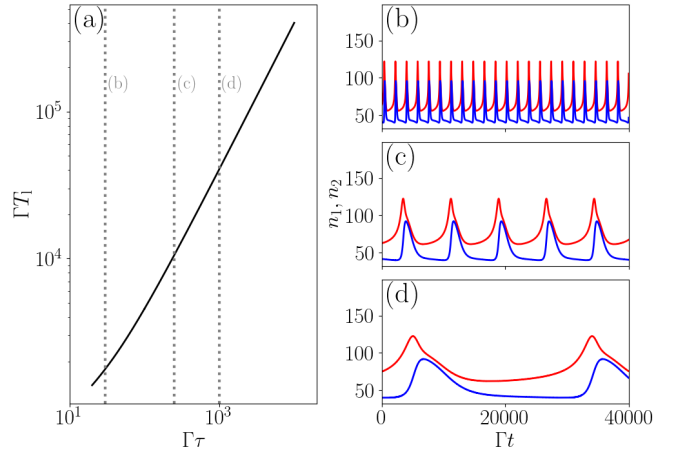
FIG. 9. (a) Limit cycle period T_1 versus memory time \tau , calculated via numerical continuation. Dotted lines indicate the memory times considered in (b)-(d). (b)-(d): n_1 (red) and n_2 (blue) versus time in a limit cycle regime for different memory times \tau . (b) \tau = 30\Gamma^{-1} . (c) \tau = 250\Gamma^{-1} . (d) \tau = 1000\Gamma^{-1} . F_1 = 15.72\sqrt{\Gamma} , F_2 = 15.68\sqrt{\Gamma} . Other model parameters are as in Fig. 6.
