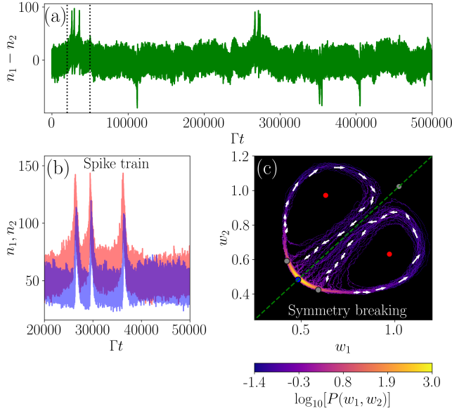
FIG. 10. (a) Intensity difference n_1 - n_2 versus time, for a standard deviation of the laser noise D = 0.55\sqrt{\Gamma} . Each spike represents an instance of spontaneous mirror symmetry breaking, whereby the intensity in one of the cavities substantially exceeds that in the other. (b) Zoom in on the first bursting event of (a) with n_1 in red and n_2 in blue. (c) Probability density function P(w_1, w_2) computed from numerical time traces. Small white arrows indicate the rotation direction of each stable limit cycle. Dots represent fixed points color coded as in Fig. 2. The dashed green line shows the axis of symmetry ( w_1 = w_2 ). Model parameters are as in Fig. 6 with F = 15.7\sqrt{\Gamma} and \rho = 0 .
