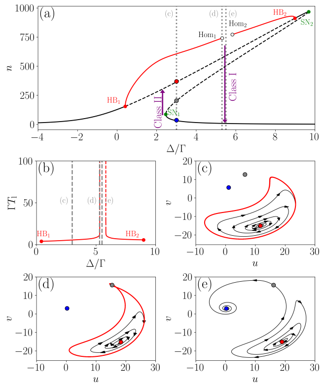
FIG. 2. (a) Intensity n as function of \Delta/\Gamma for F = 22\sqrt{\Gamma} . Solid (dashed) black curves correspond to stable (unstable) fixed points. Green and red dots indicate saddle-node ( SN_i ) and Hopf ( HB_i ) bifurcations, respectively. Red solid curves show the maximum n of limit cycle oscillations. Open black circle indicates homoclinic bifurcations ( Hom_i ). Purple arrows indicate transition directions with associated classes shown in Fig. 3. (b) Period of the limit cycle oscillations, T_l , as function of \Delta/\Gamma . (c,d,e) Phase portraits at the detunings indicated by the dashed gray lines in (b). Dots indicate fixed points, with blue, red and gray corresponding to stable focus, unstable focus, and saddle, respectively. Black curves show orbits with arrows indicating the direction. Red curves show stable limit cycles. Model parameters are as in Fig. 1, with \Delta = 3\Gamma , \Delta = 5.3\Gamma , and \Delta = 5.5\Gamma in (c), (d) and (e), respectively.
