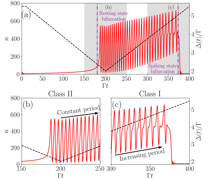
FIG. 3. n (solid red curve, left vertical axis) and detuning \Delta/\Gamma (dashed black line, right vertical axis) versus time \Gamma t . (a) Shaded areas correspond to the close-up views [(b)-(c)] of the transition from resting to spiking states, or vice versa, located by dashed-dotted vertical purple lines. (b) Zoom in on the resting state bifurcation corresponding to class II excitability in Fig. 2(a). (c) Zoom in on the spiking state bifurcation associated with class I spiking in Fig. 2(a). Model parameter values are as in Fig. 2(a). The detuning varies between \Delta = 5.5\Gamma and \Delta = 2.2\Gamma .
