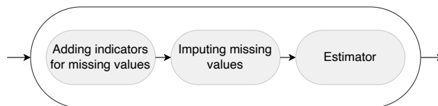
Figure 1: Generic pipeline for training and evaluating the classification model.
