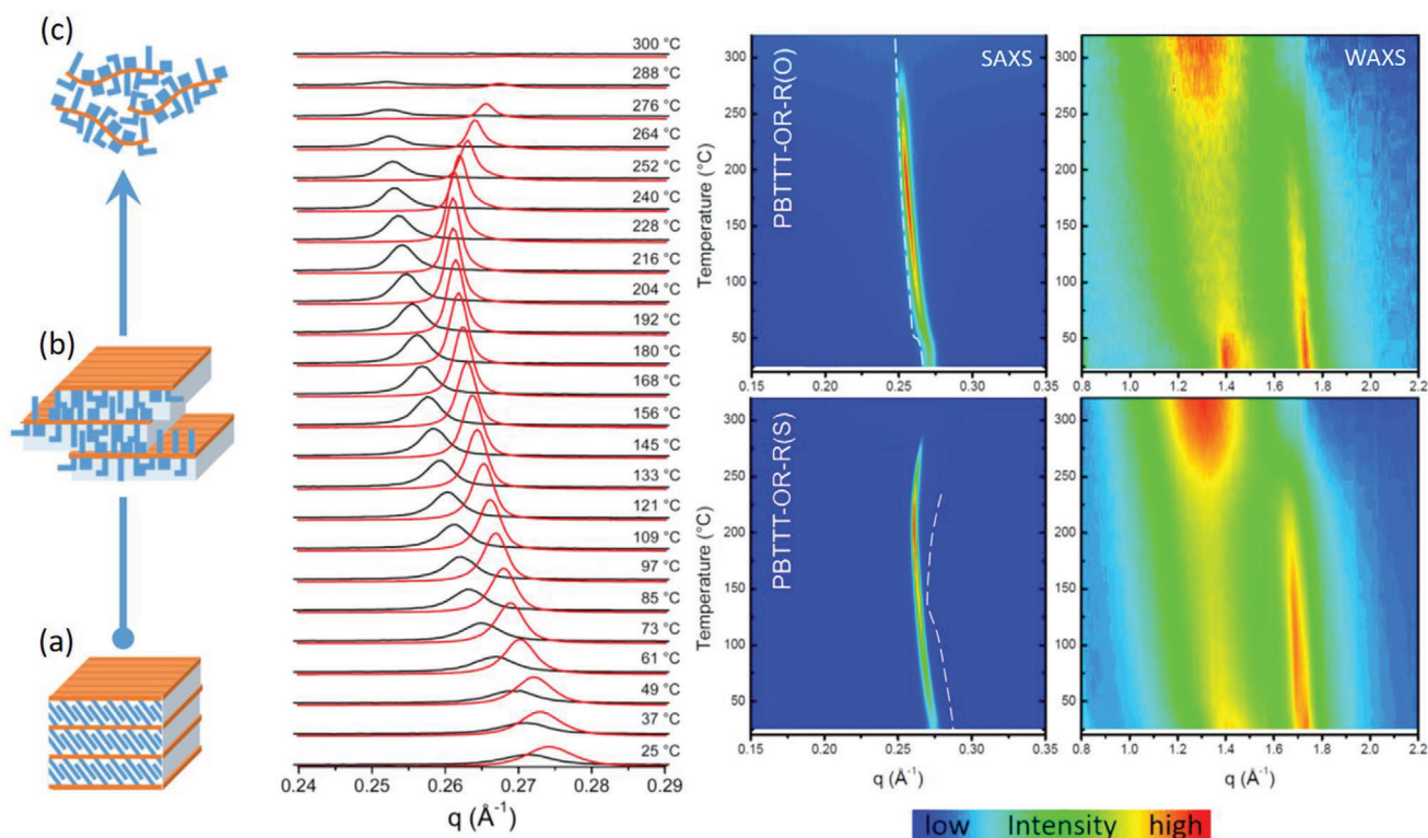
Figure 6. Selected temperature-resolved SAXS patterns of PBTTT-OR-R(O) (black) and PBTTT-OR-R(S) (red) and all top-viewed color-coded SAXS/WAXS data during heating at 50 K min -1 after cooling at 20 K min -1 for PBTTT(O) and after cooling at 5 K min -1 for PBTTT(S) (top panels: SAXS and WAXS of PBTTT-OR-R(O); bottom panels: SAXS and WAXS of PBTTT-OR-R(S)). Left: Schematic representation of conversion from the crystalline a) to the sanidic liquid crystalline state b) by side chain (blue lines) melting, followed by backbone (orange lines) melting into the fully molten state c). The dashed white lines in the colored SAXS panels of PBTTT-OR-R(O) and PBTTT-OR-R(S) are from PBTTT-(OR) 2 (O) and PBTTT(S), respectively (for comparison). [17]
