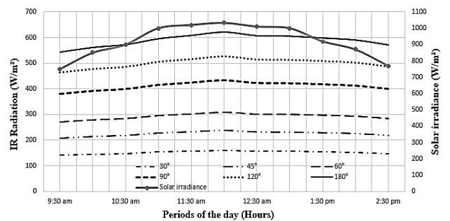
Figure 12. IR radiation absorbed by the W-shape collector for different angle values of the W absorber
