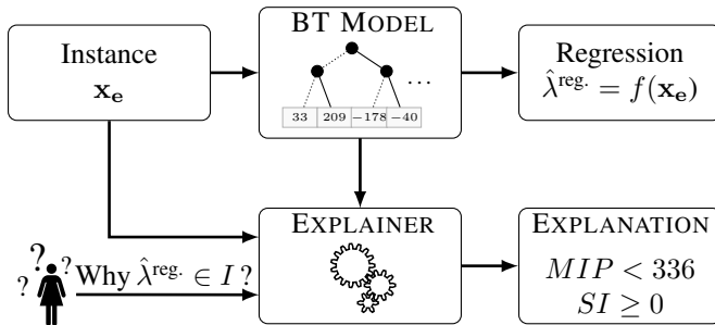
Fig. 2: Flowchart of the logic-based explainable method
