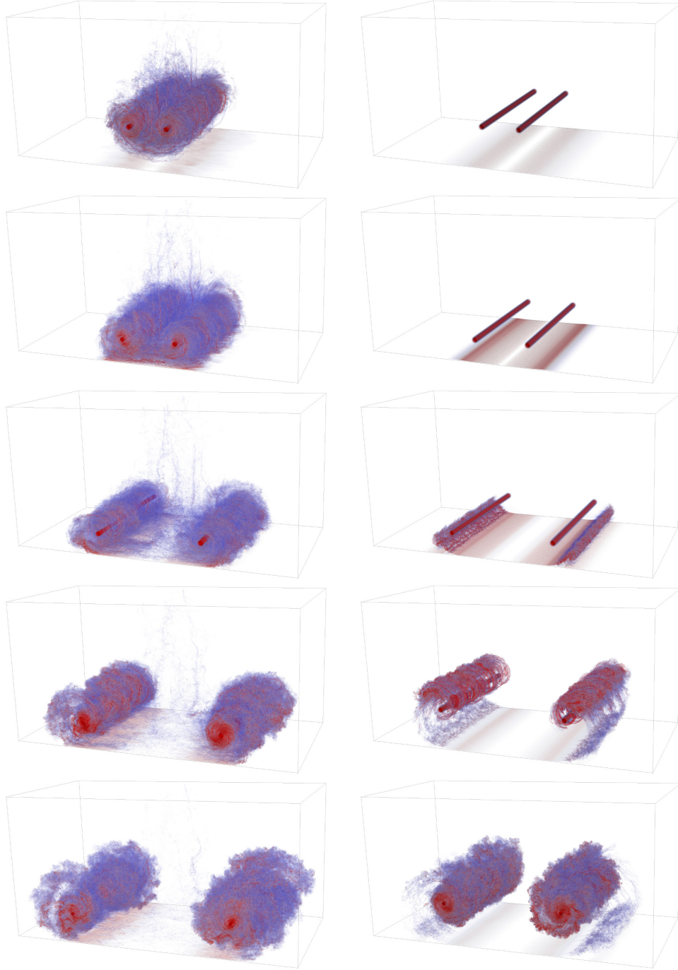
Figure 6: Volume rendering of the vorticity magnitude at t/t_0 = 1, 2, 3, 4, 5 : T-2VS (left) and BH-2VS (right).
