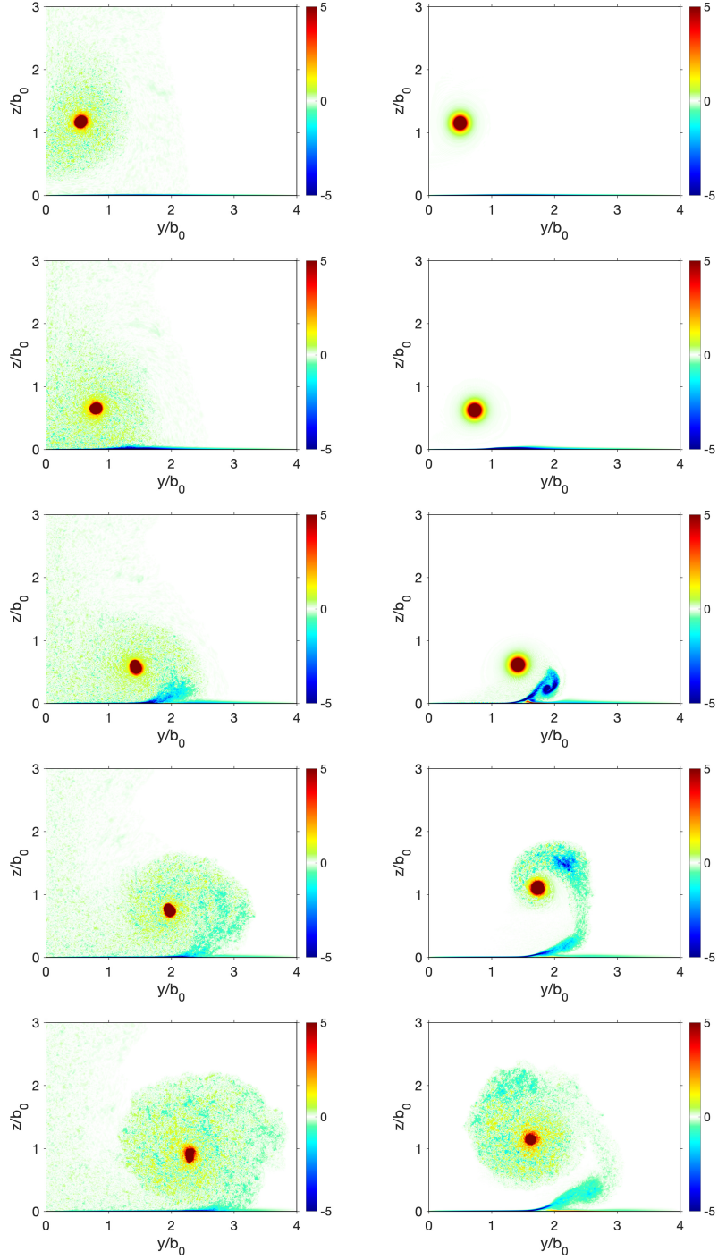
Figure 7: Mean axial vorticity, \langle \omega_x \rangle b_0^2 / \Gamma_0 , at t/t_0 = 1, 2, 3, 4, 5 : T-2VS (left) and BH-2VS (right).
