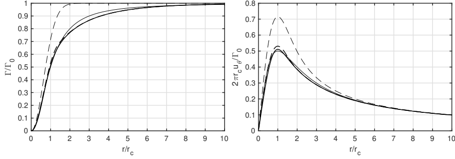
Figure 1: Circulation (left) and induced velocity (right) profiles for various wake vortex models: single scale models: BH (thin solid) and LO (thin dash); two-scale models for the case r_c/b_0 = 0.050 : P (dash) and PW (solid).
