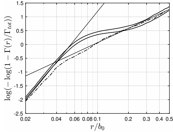
Figure 5: Analysis of the outer and inner scalings for the circulation distributions: T-2VS of Case 0 (solid); partially completed rollup ( t/t_0 \approx 1 ) of a wake started using five-hole probe measurements of the velocity field just behind a large A340-type generic model in landing configuration (dash-dot; using simulation data by UCLouvain in the AWIATOR project). The straight lines indicate the slope 2 and the slope q = 0.75 (here \beta_o \approx 6.0 ).
