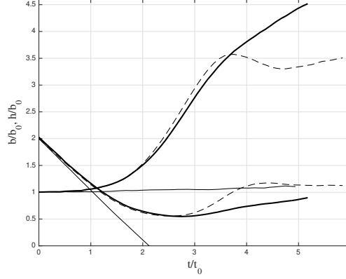
Figure 10: Evolution of the vortex height h/b_0 and of the vortex spacing b/b_0 : T-2VS (thick solid) and BH-2VS (dashed). The evolutions for the T-2VS evolving OGE is also shown for comparison (thin solid).
