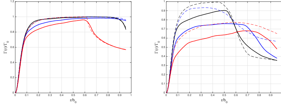
Figure 15: Vortex circulation distribution at t/t_0 = 0 (black), 1 (blue) and 2 (red) on the left, and at t/t_0 = 3 (black), 4 (blue), 5 (red) on the right, for the T-2VS (thick solid) and for the BH-2VS (thin dashed).
