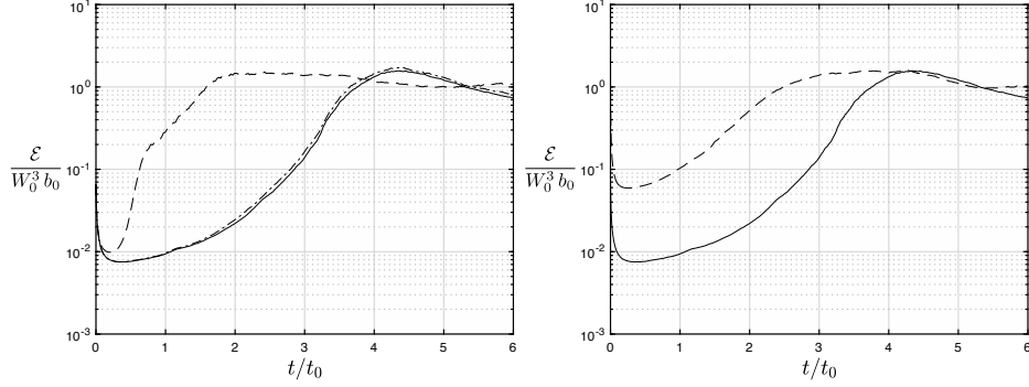
Figure 3: Evolution of the dimensionless energy dissipation rate. Left: baseline BH-2VS (Case 0, solid), PW-2VS (Case 1, dashed-dotted) and LO-2VS (Case 2, dashed), all with very weak HIT. Right: BH-2VS with very weak HIT (Case 0, solid) and with HIT of ten times higher dissipation rate (Case 3, dashed).
