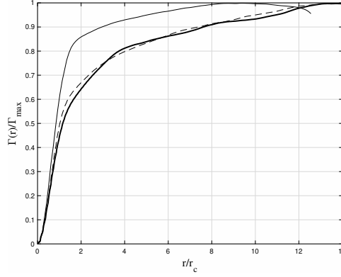
Figure 16: Circulation distribution at late times: T-2VS at t/t_0 = 5 (thick solid) and BH-2VS at t/t_0 = 5.9 (dashed). The circulation distribution of the T-2VS OGE is also recalled for comparison (thin solid).
