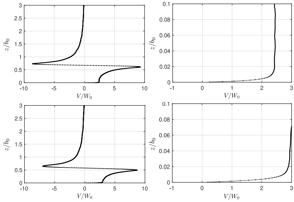
Figure 9: Profiles of the longitudinally averaged velocity component V for the T-2VS: t/t_0 = 1.9 and y/b_0 = 0.78 (top), t/t_0 = 3.0 and y/b_0 = 1.46 (bottom). A zoom near the ground is also provided (right). The dots correspond to the location of the grid points.
