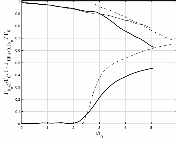
Figure 14: Evolution of the vortex circulation \Gamma_{b_0/2} (top curves) and of the separated secondary vorticity \Gamma_0 - \Gamma_{HP|z>0.1b_0} (bottom curves): T-2VS (thick solid) and BH-2VS (dashed). The evolution of \Gamma_{b_0/2} for the T-2VS evolving OGE is also shown (thin solid).
