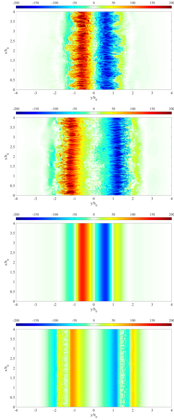
Figure 8: Axial vorticity at the wall, \omega_x b_0^2/\Gamma_0 , at t/t_0 = 2 and 3: T-2VS (top) and BH-2VS (bottom).
