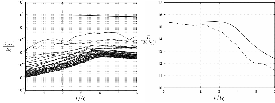
Figure 2: Evolution of the kinetic energy for the baseline Case 0. Left: longitudinal modal energy: mean flow (thick solid), mode \lambda = 4b_0 (solid), and next 31 modes (thin solid) down to \lambda = 0.125b_0 . Right: total energy E (solid) and mean flow energy E_{2D} (dashed).
