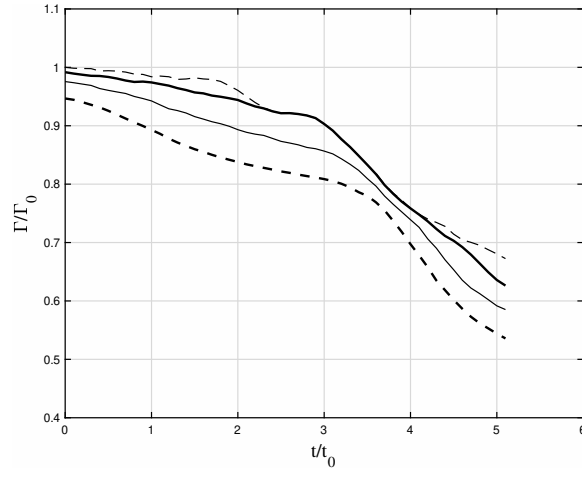
Figure 12: Evolution of the various vortex circulation diagnostics for the T-2VS: \Gamma_{max} (thin dash), \Gamma_{b_0/2} (thick solid), \Gamma_{15} (thin solid) and \Gamma_{5-15} (thick dash).
