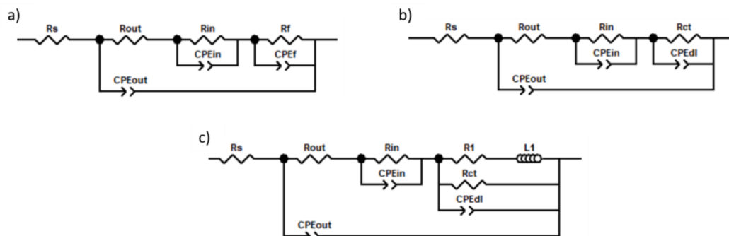
Fig. 13. Equivalent circuits for the fitting of EIS data.
