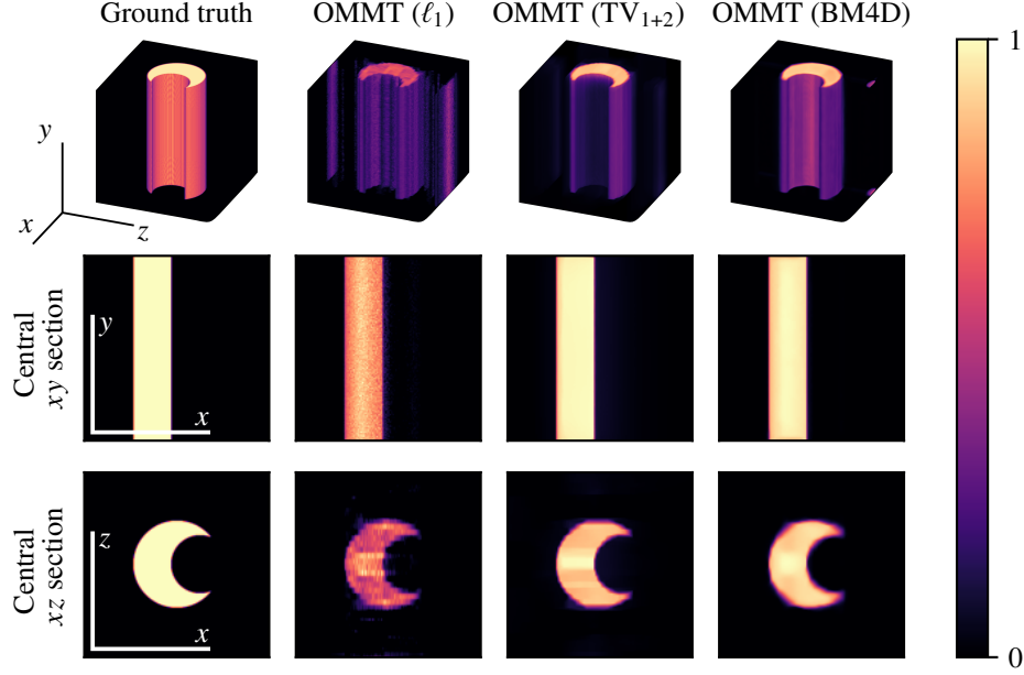
Fig. 4. Reconstruction of a simulated sample using the different regularization priors. The \ell_1 result contains more noise and has fuzzy edges in the xz section, while TV_{1+2} and BM4D give a much smoother result with better defined edges. 3D views use attenuated mean intensity projection. Scale bar axes are 50\ \mu\text{m} .
