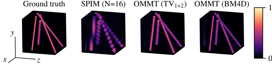
Fig. 6. Volumetric reconstructions on simulated objects in a noisy scenario compared to an undersampled SPIM with equal phototoxicity. OMMT reconstructions are smoother, with a minor improvement when using BM4D over TV 1+2 . Attenuated mean intensity projection is shown, and axes are 50 \mu m scale bars.
