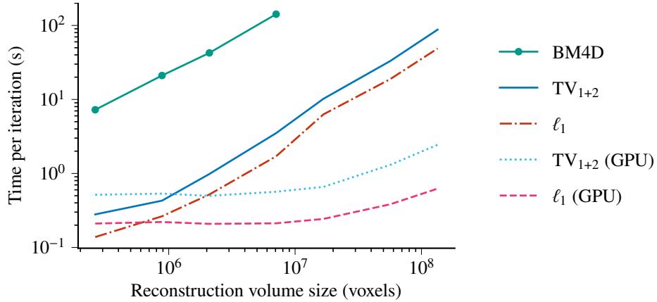
Fig. 7. Average time per iteration of our ADMM optimization loop for different regularization priors. BM4D is not realistically useable to reconstruct big images, but both TV_{1+2} and \ell_1 are fast enough to be applied to real size experimental data. This is particularly true with the 30\times speed-up when running with GPU acceleration. See Table 2 for detailed values.
