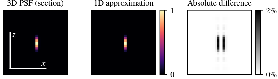
Fig. 2. Comparison of a full simulated light sheet PSF and its 1D approximated model, represented as a 1D manifold in 3D space. Since the lateral extent of the PSF is negligible with respect to its axial one, the maximum difference between the two is lower than 2 %. Scale bar axes are 10 \mu\text{m} .
