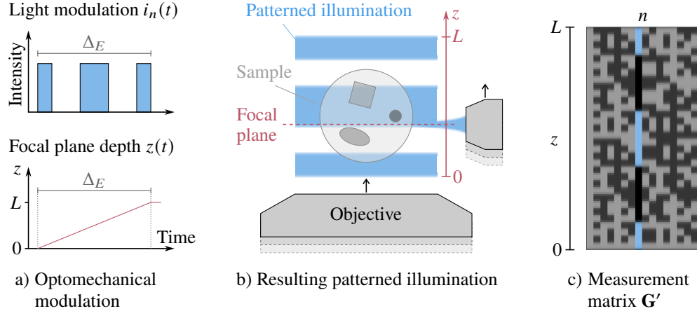
Fig. 1. Overview of OMMT imaging. (a) Optomechanical modulation combines focus sweeping synchronized with temporal light modulation. (b) The modulation creates a patterned illumination in the depth axis. (c) This is repeated to acquire N projections with different modulation functions, which are stacked into the measurement matrix G' .
