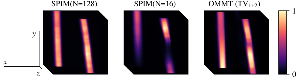
Fig. 9. OMMT reconstruction of fluorescent textile fibres and comparison to undersampled SPIM, with a larger depth span of 800\text{ }\mu\text{m} . Information located between sampled planes is missing in the undersampled SPIM volume, where no gaps are present in the \text{TV}_{1+2} image. Views use mean intensity projection, and axes are 100\text{ }\mu\text{m} scale bars.
