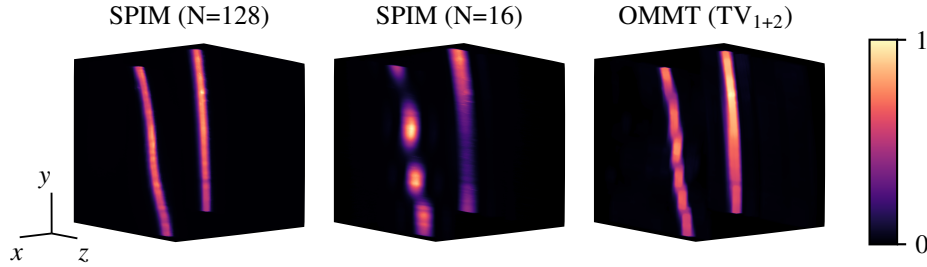
Fig. 8. OMMT reconstruction of fluorescent textile fibres and comparison to undersampled SPIM with equal light dose. The reconstructed image with TV_{1+2} prior is smoother, and looks similar to the reference SPIM volume. Views use mean intensity projection, and axes are 100\ \mu\text{m} scale bars.
