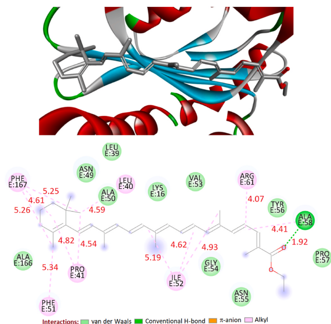
Fig. 6. The binding interactions of 2 against P. aeruginosa LasR (PDB: 2UV0).
