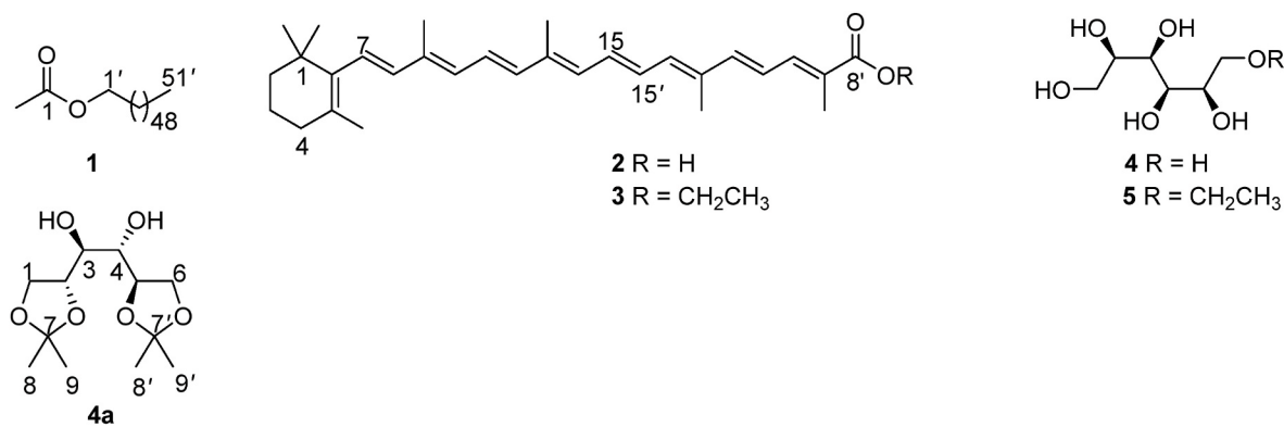
Fig. 1. Chemical structures of compound 1–5.
