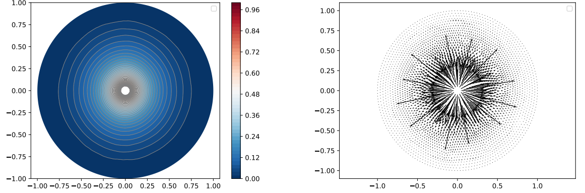
Figure 3: An annulus and a nonsmooth \rho : 20 level lines (left) and a gradient map (right)
