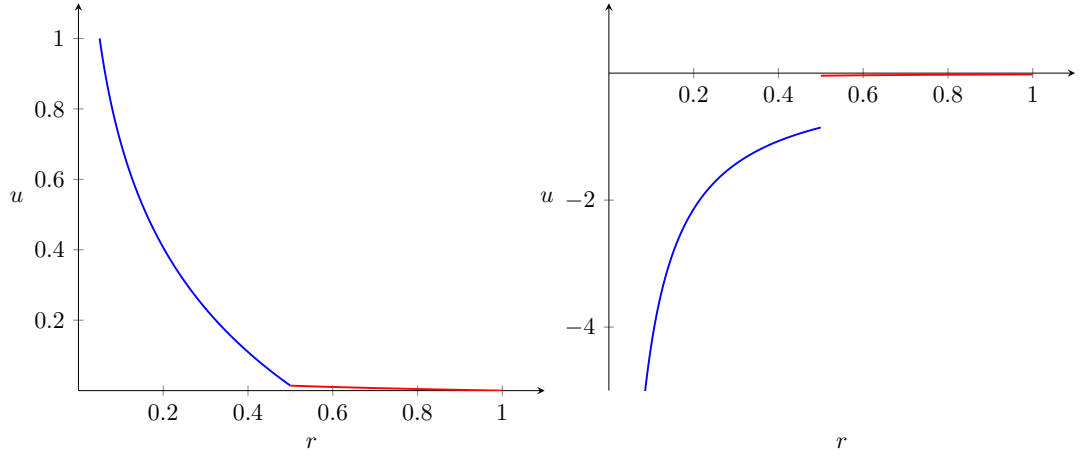
Figure 9: The solution u (left) and \frac{\partial u}{\partial r} (right) with respect to r for a radially discontinuous coefficients
