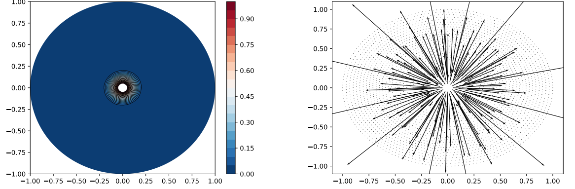
Figure 10: An annulus with a piecewise constant \rho (discontinuous far from the interior boundary): 20 level lines (left) and a gradient map (right)
