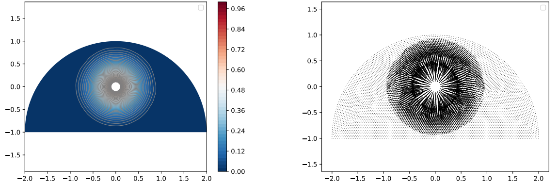
Figure 6: A half-disc with 1 hole and a smooth \rho : 20 level lines (left) and a gradient map (right)
