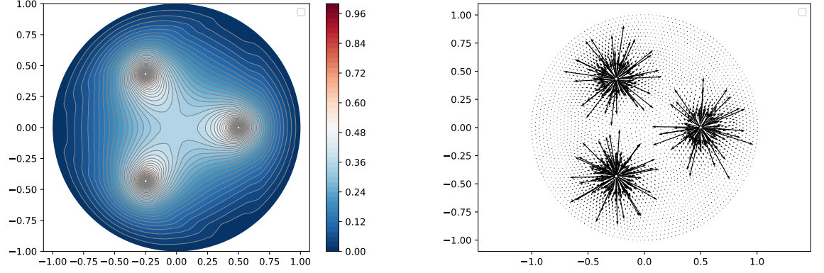
Figure 5: The unit ball with 3 holes and a degenerate \rho : 20 level lines (left) and a gradient map (right)
