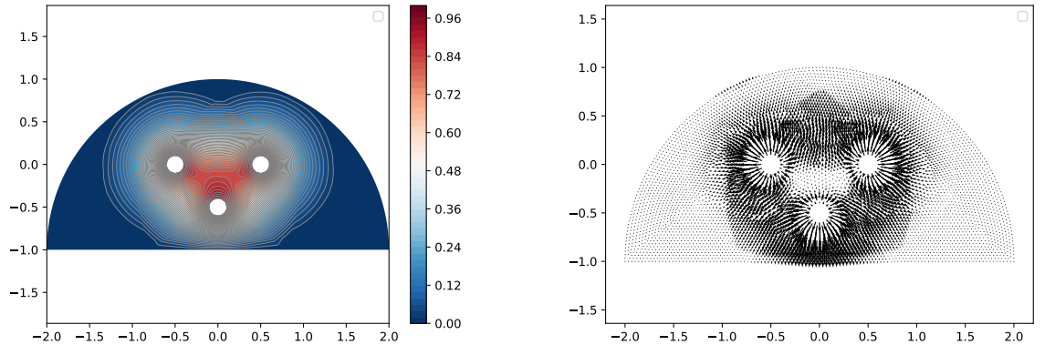
Figure 8: A half-disc with 3 holes and a smooth \rho : 20 level lines (left) and a gradient map (right)
