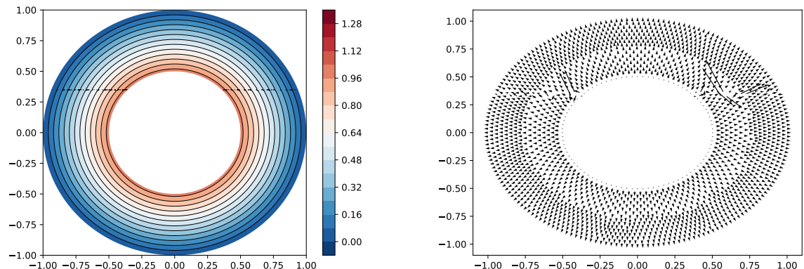
Figure 11: An annulus with a piecewise constant \rho (discontinuous line cuts the interior boundary): 20 level lines (left) and a gradient map (right)
