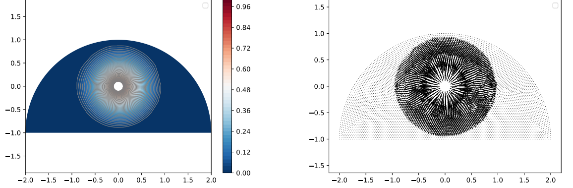
Figure 7: A half-disc with 1 hole and a degenerate \rho : 20 level lines (left) and a gradient map (right)
