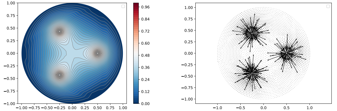
Figure 4: The unit ball with 3 holes and a smooth \rho : 20 level lines (left) and a gradient map (right)
