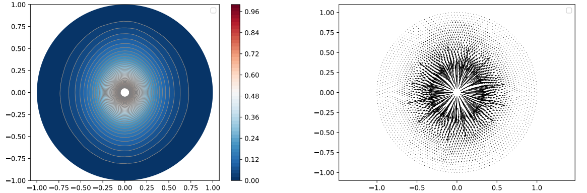
Figure 2: An annulus and a smooth \rho : 20 level lines (left) and a gradient map (right)
