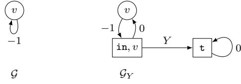
Fig. 5 An example where the operator \mathcal{H} is not Scott-continuous.
