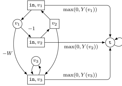
Fig. 4 MCR game \mathcal{G}_Y associated with the total-payoff game of Fig. 2
