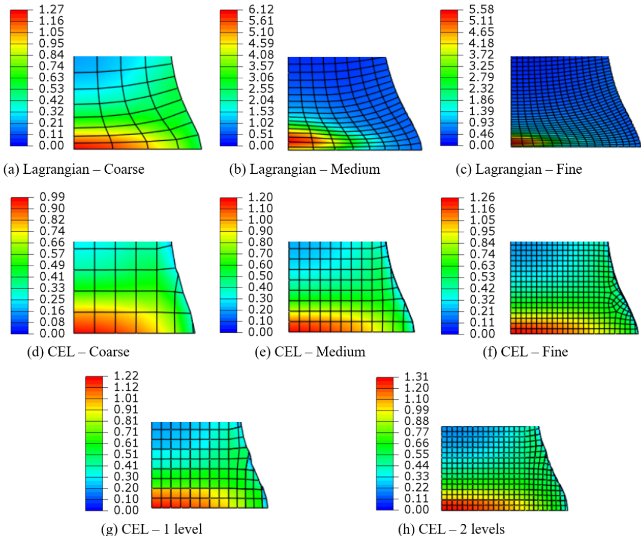
Fig. 5. End of the deformed specimen results showing the mesh and the equivalent plastic strains for the Lagrangian coarse (a), Lagrangian medium (b), Lagrangian fine (c), CEL coarse (d), CEL medium (e), CEL fine (f), and CEL adaptive mesh refinement with 1 level (g) and 2 levels (h) meshes
