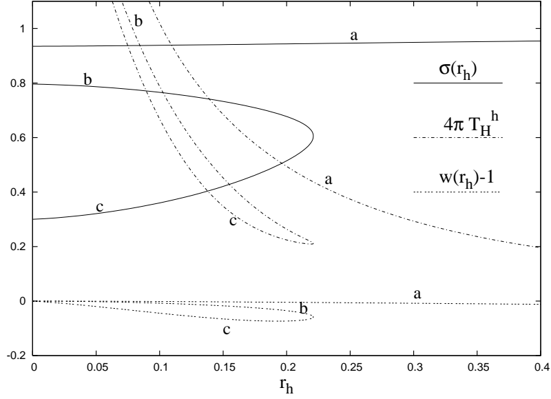
Figure 7. The event horizon Hawking temperature, the value of the gauge potential on the event horizon w_h as well as the value of the metric function \sigma at the event horizon, are shown as functions of the event horizon radius for d = 5 black hole solutions of F(2) + F(4) theory with \alpha^2 = 0.25 , \Lambda = 0.0004 .
