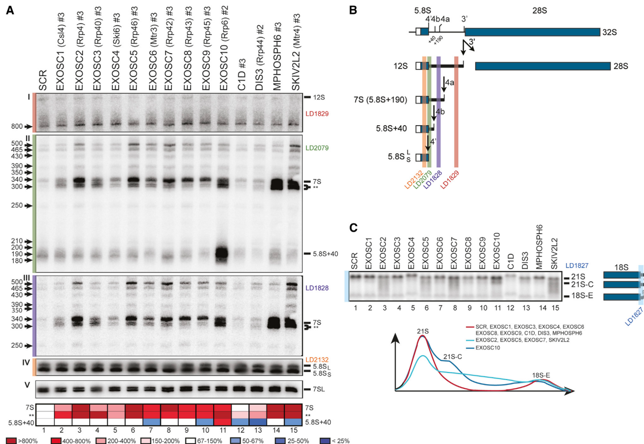
Figure 6. Involvement of Individual Subunits of the Human RNA Exosome in Pre-rRNA Processing of ITS1 and ITS2
